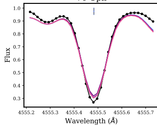
10 Tau
