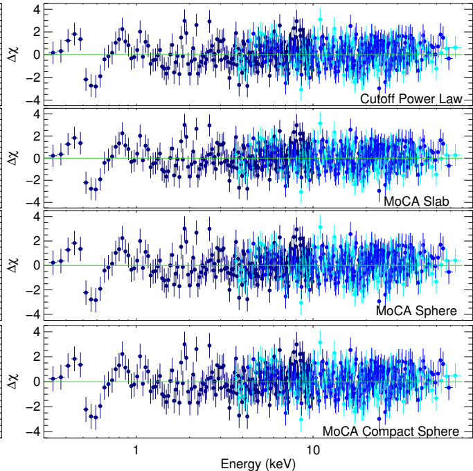
XMM-NuSTAR 2014 best fit residuals
