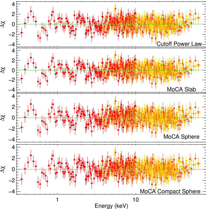
XMM-NuSTAR 2013 best fit residuals
