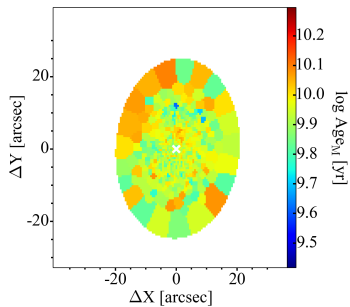
J-PLUS/MUFFIT
