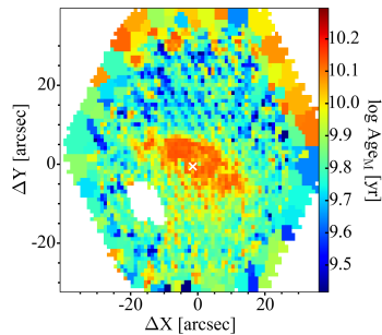
CALIFA/STARLIGHT
