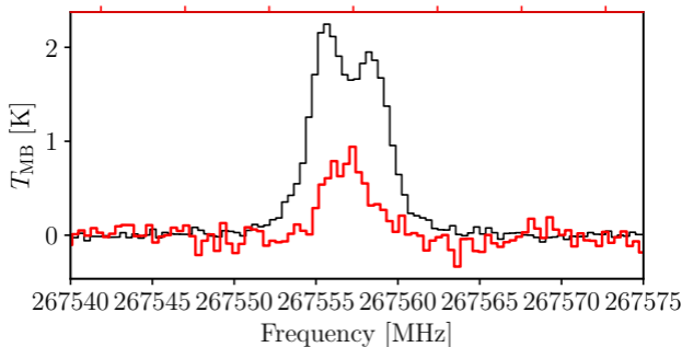
Clump 2, \text{HCO}^+ , 3 \times \text{H}^{13}\text{CO}^+
