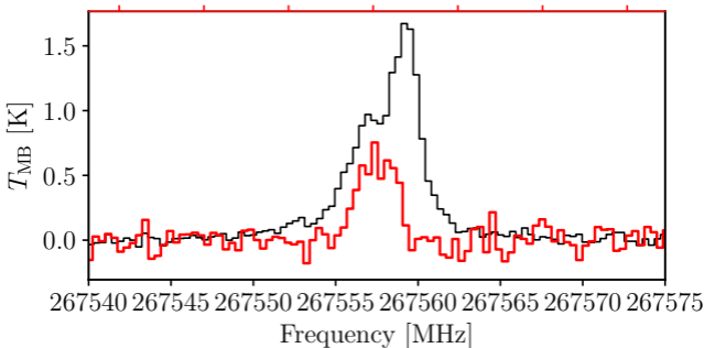
Clump 5, \text{HCO}^+ , 3 \times \text{H}^{13}\text{CO}^+
