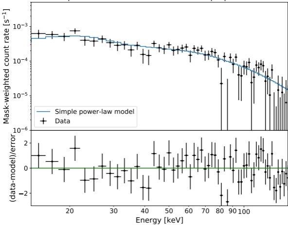
BAT spectrum for the T100 interval with simple power-law fit
