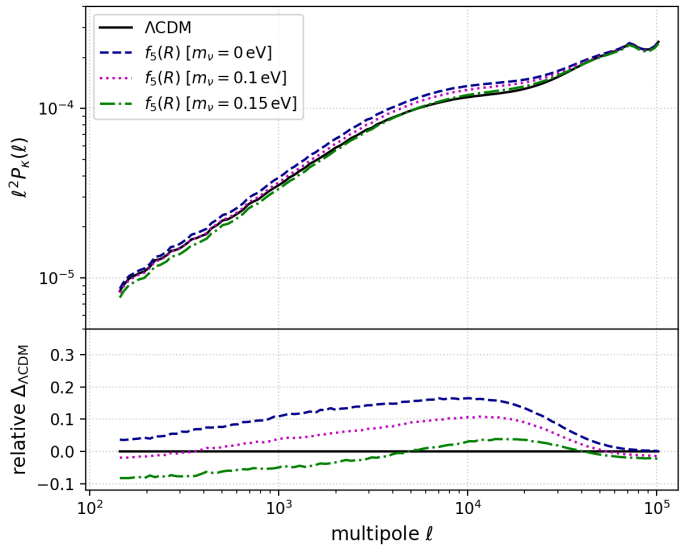
source redshift z_s = 2.0
