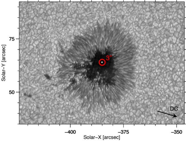
NOAA12149, 2014-08-25 T 10:36 UTC, Gband context image
