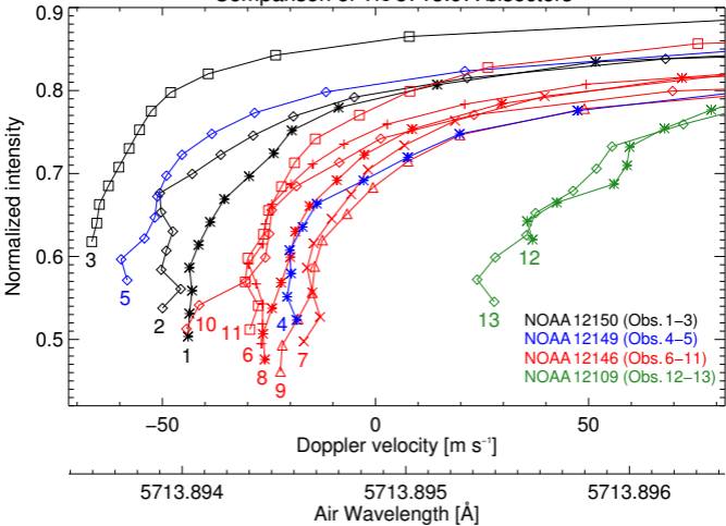
Comparison of Ti I 5713.9Å bisectors
