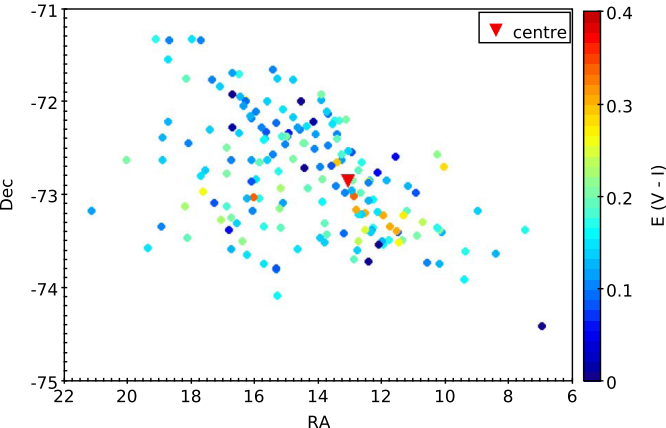
Reddening distribution
