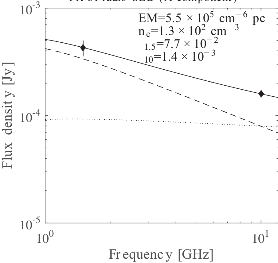
Fit of radio SED (A component)
