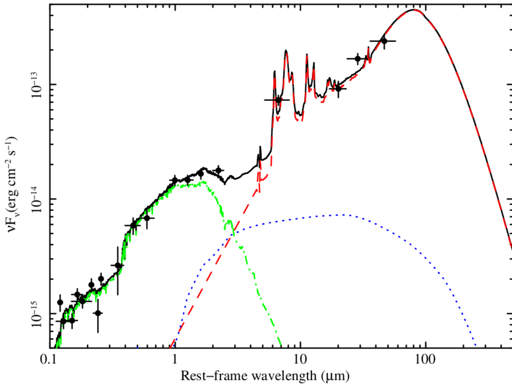
SRC 309 – z=2.579
