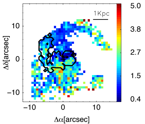
EW_{NaD}
