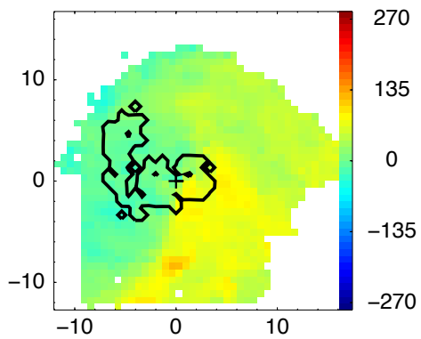
V_{H\alpha}
