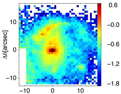
Continuum
