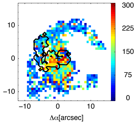
\sigma_{NaD}
