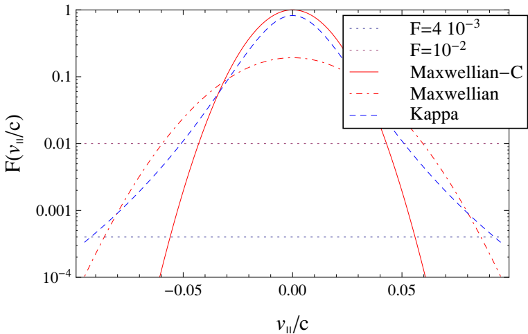
(a) – VDFs in parallel direction
