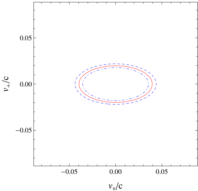
(c) – Contours of VDFs at F(v_{\parallel}/c)=2 \cdot 10^{-2}
