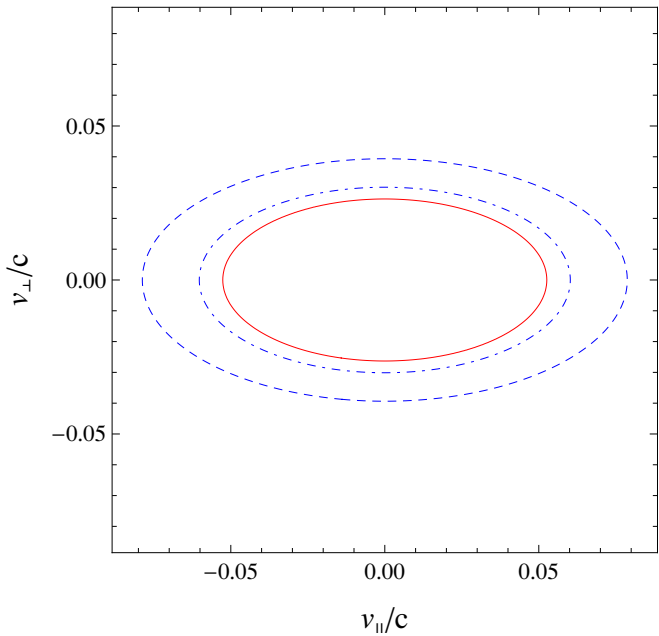
(b) – Contours of VDFs at F(v_{\parallel}/c)=10^{-3}
