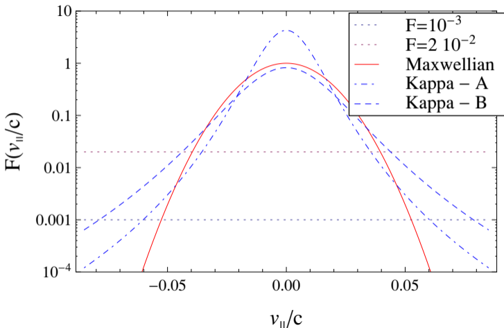
(a) – VDFs in parallel direction
