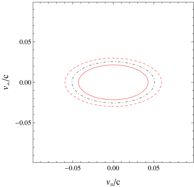
(c) – Contours of VDFs at F(v_{\parallel}/c)=10^{-2}
