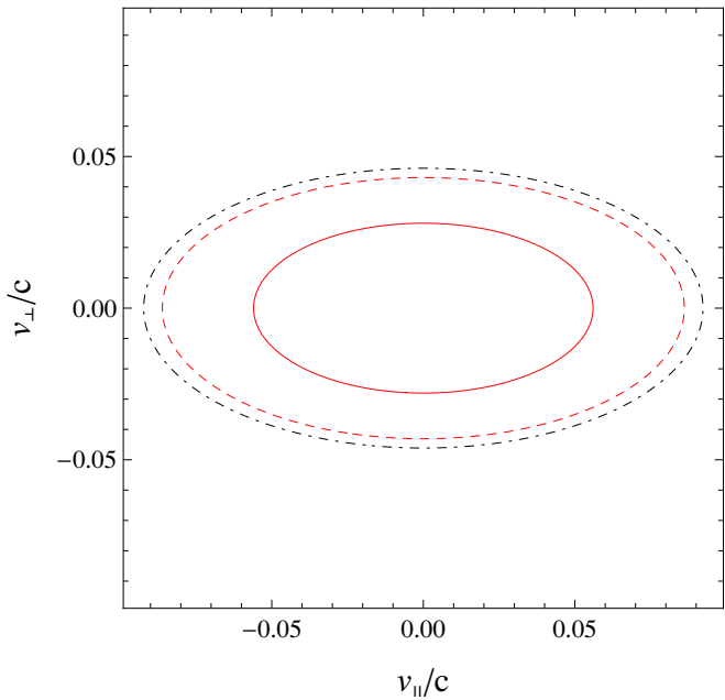
(b) – Contours of VDFs at F(v_{||}/c)=4 \cdot 10^{-4}
