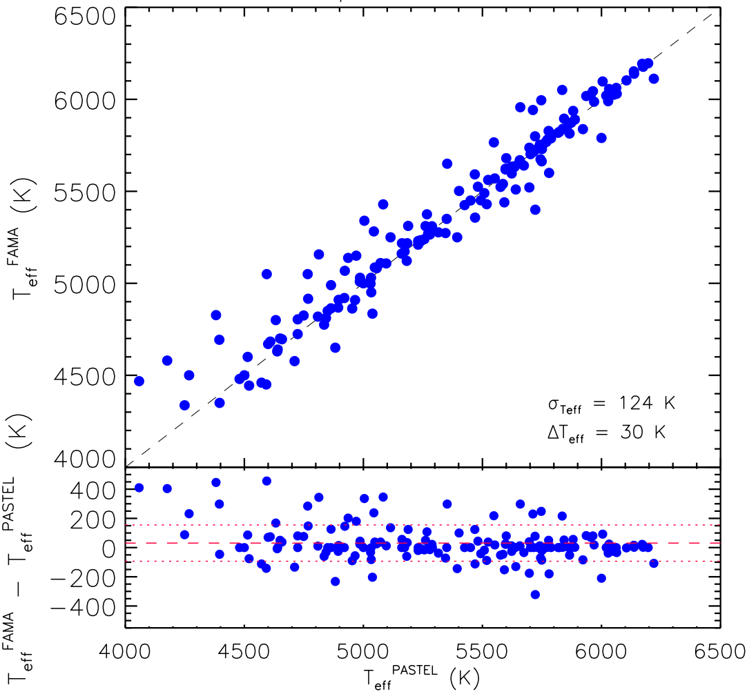
Elodie Templates: FAMA vs PASTEL
