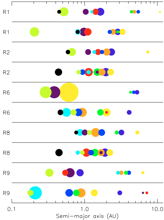
Fig. 8. Snapshots of two randomly selected simulations from the model classes shown, with the exception of the first (R1) and fourth (R2) rows, which correspond to Figs. 7 and 9 respectively. The snapshots are taken at t = 2 \times 10^5 yrs. The area of each planet is linearly proportional to its mass; the smallest body (in the top row) is of 2 M_{\oplus} , and the largest (formed from multiple collisions) is of 39 M_{\oplus} . The co-orbitals of Fig. 9 are clearly visible as concentric circles. (The figure is available in colour in the online version.)
