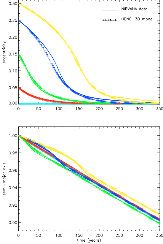
Fig. 1. (Top) Eccentricity evolution of a 10 M_{\oplus} protoplanet on a variety of eccentric orbits. Solid lines are the results from NIRVANA, crosses from the N -body code. (Bottom) The corresponding migration rates. (The figure is available in colour in the online version.)
