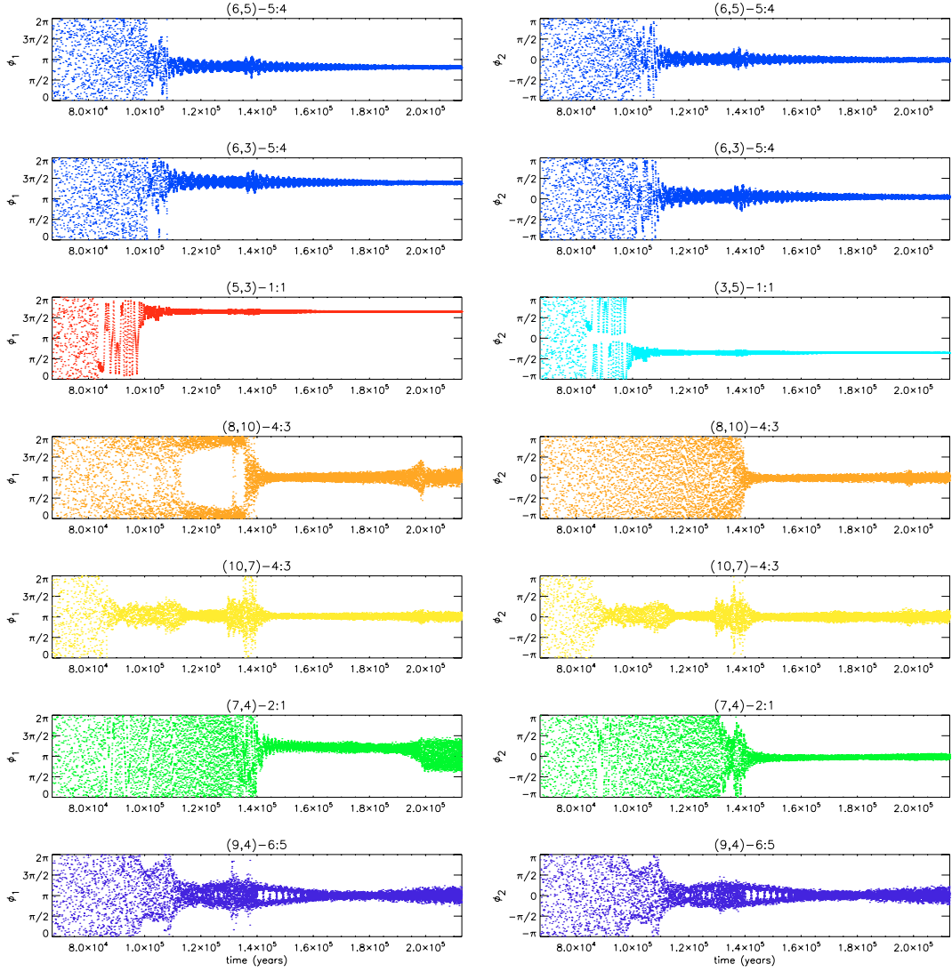
Fig. 6. The first order mean-motion resonances between the planets in Fig. 5, during the longest resonant migration phase. Each plot is labelled (P_i, P_j)-p:q , where P_i and P_j are the exterior and interior protoplanets in each resonance respectively, and p:q is the commensurability between them. (The figure is available in colour in the online version.)
