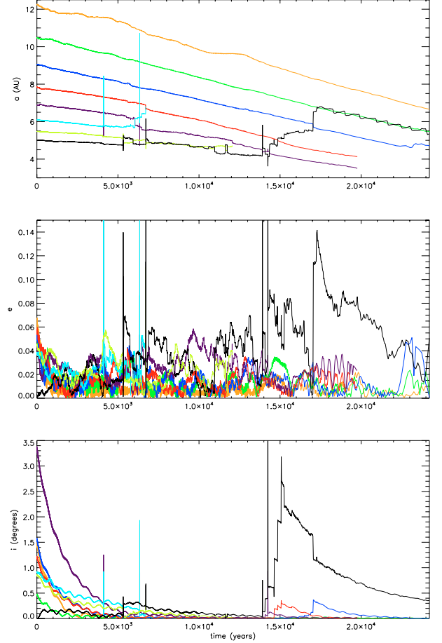
Fig. 4. Orbital elements for the 3D NIRVANA model, similar to Fig. 5 but with eight protoplanets (run H1). Behaviour is similar to the early stages of the N -body models, with scattering and collisions among the inner population. A co-orbital system is formed, which remains stable for the remainder of the integrations. Note only the smallest protoplanet achieves e > 0.1 or i > 0.5^\circ after the initial values have been damped. The 6 and 10 M_{\oplus} protoplanets collide at t = 6.7 \times 10^3 yrs, and the 4 and 8 M_{\oplus} protoplanets collide at t = 1.20 \times 10^4 yrs. (The figure is available in colour in the online version.)
