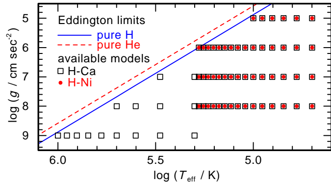
Fig. 3. Parameters of available NLTE model atmosphere fluxes. The H-Ni models are limited to T_{\text{eff}} \leq 190 kK because Kurucz's line lists (1996) provide only data up to ionization stage IX.
