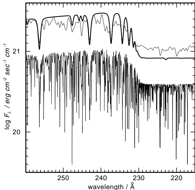
Fig. 2. Comparison of NLTE model atmosphere fluxes ( T_{\text{eff}} = 130 kK, \log g = 7 , solar abundances) without (thick line) and with consideration of iron-group opacities. For clarity, the spectra are convolved with a Gaussian of FWHM = 0.5 Å (the original H-Ni flux is shown in addition, shifted down by 0.5 dex).
