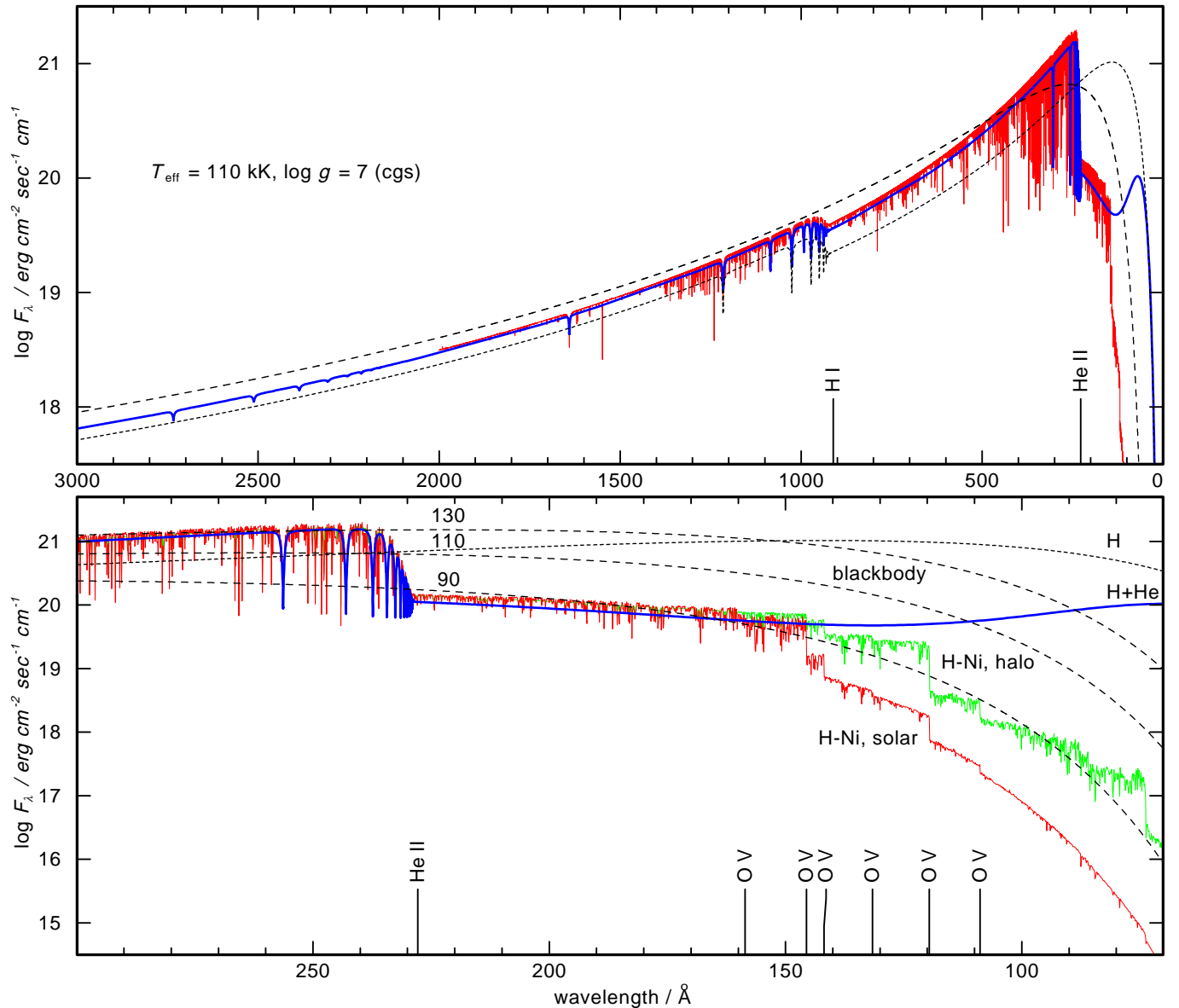
Fig. 1. Top: comparison of NLTE model atmosphere fluxes ( T_{\text{eff}} = 110 \text{ kK} , \log g = 7 ) calculated with different chemical composition. Short dashes: pure H model, thick line: H+He, thin line: H-Ni with [Z] = 0 . Note that the main deviations of the blackbody (long dashes, 110 kK) to the synthetic spectra occur shortwards of the indicated H I and He II ground state thresholds. Lower panel: Detail of the upper panel; in addition, a H-Ni model with [Z] = -1 (thin line), and three blackbody fluxes (long dashes, 90, 110, 130 kK) are shown. The prominent He II and O V absorption edges are indicated. Note the drastic decrease of the flux level at shorter wavelengths, if the opacities of metals are considered.
