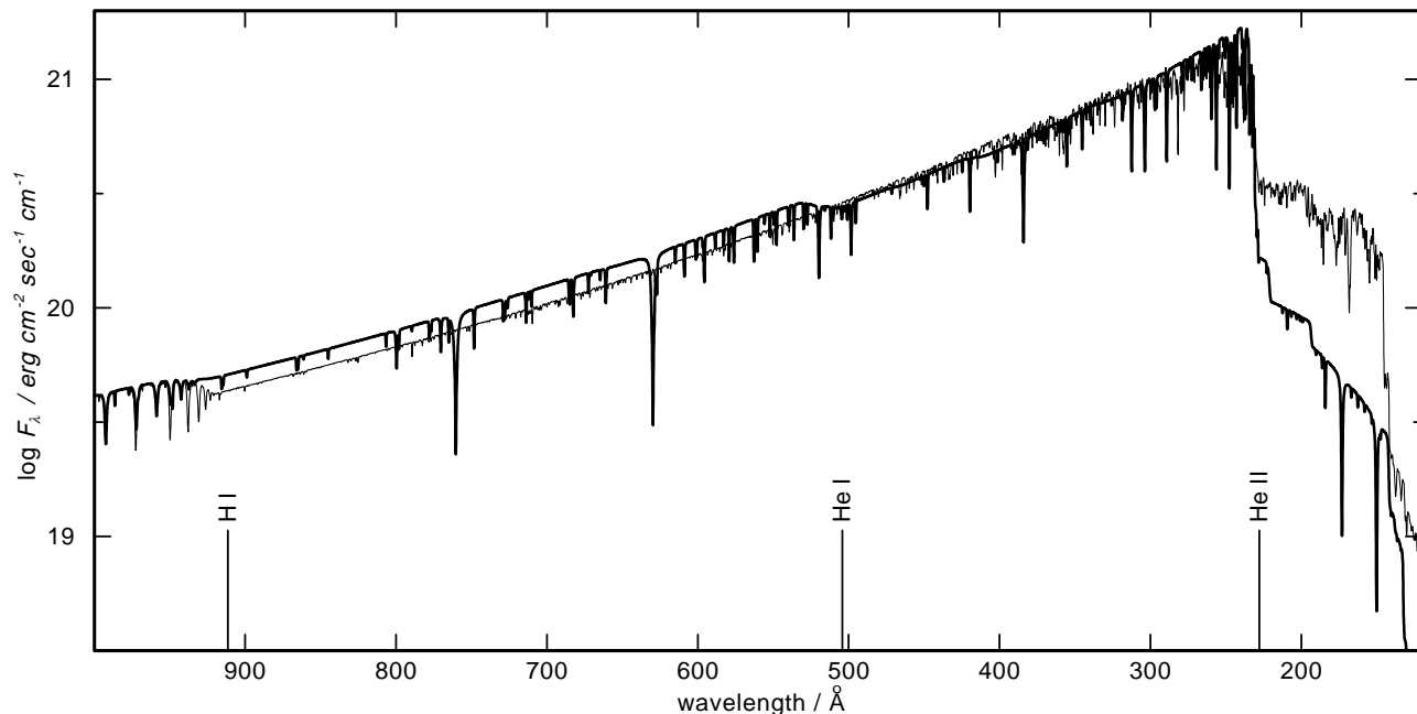
Fig. 5. Comparison of NLTE model atmosphere fluxes ( T_{\text{eff}} = 110 \text{ kK} , \log g = 6 ) calculated with a solar (H-Ni, thin line) and a hydrogen-deficient (He:C:N:O = 33:50:2:15 by mass, thick line) composition. Note the strong differences at energies higher than the indicated H I, He I, and He II ground state thresholds). For clarity, the spectra are convolved with a Gaussian of FWHM = 0.5 \text{ \AA} .
