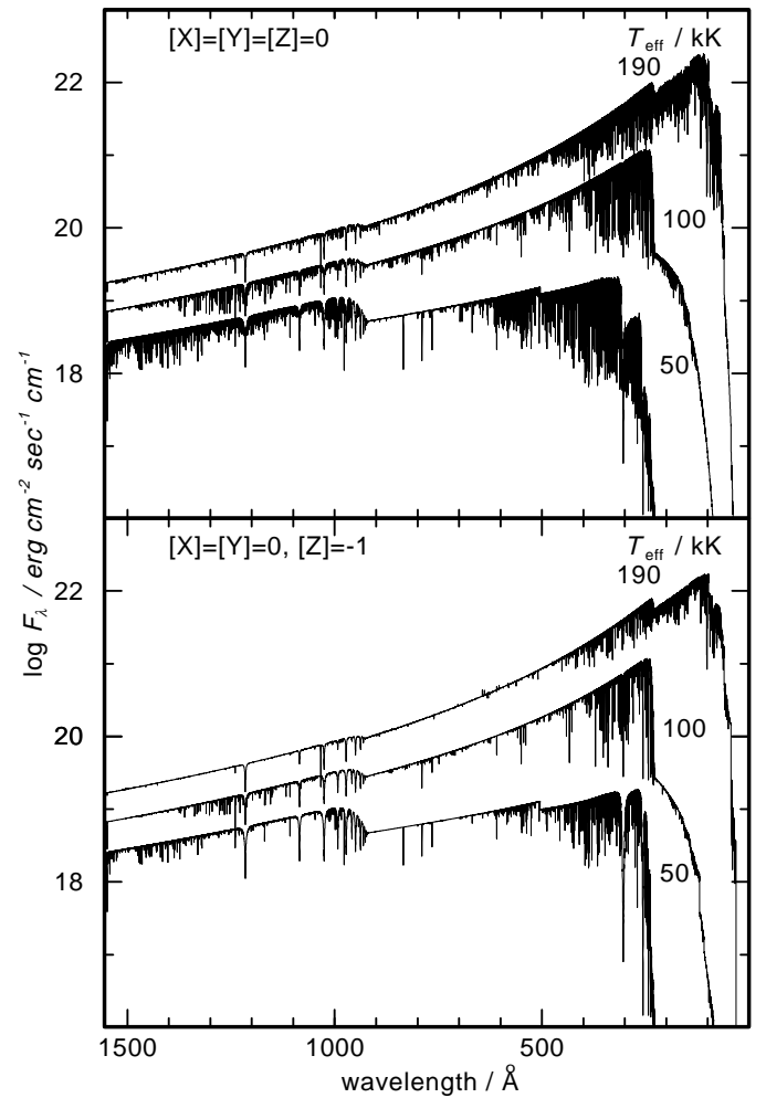
Fig. 4. Comparison of NLTE model atmosphere fluxes ( \log g = 7 ) calculated with solar (top) and halo (bottom) abundance ratios at three different temperatures.
