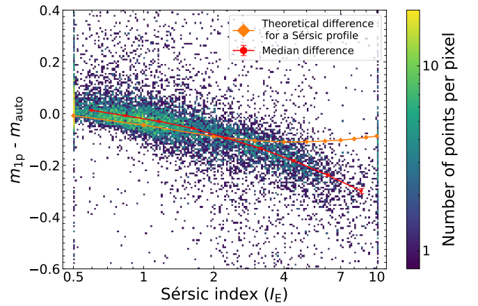
Fig. 11. Difference between the I_E single-Sérsic model magnitude m_{1p} and the adaptive aperture magnitudes m_{\text{auto}} as a function of the corresponding Sérsic index fitted in the I_E band for the 12 786 galaxies with I_E \leq 23 . Red points show the median value of that difference in bins of n as well as the associated bootstrap uncertainty. The solid orange line represents the expected magnitude difference for a pure Sérsic luminosity profile. The difference is smaller than expected for disc-like galaxies ( n \leq 1.5 ), and hence models are fainter than expected, which could be due to the model missing the excess of flux from a small and faint bulge or secondary features (e.g. spiral arms, bars, rings, flocculence). For higher Sérsic indices, the trend inverts itself, with model photometry being brighter than the adaptive aperture measurement.
