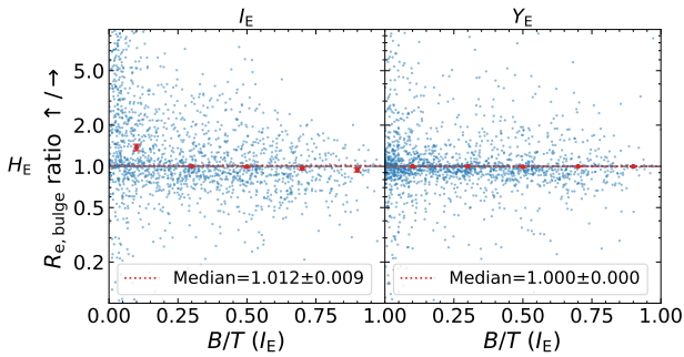
Fig. 18. Ratios of the effective radii of galaxy bulges between different VIS and NISP bands as a function of B/T measured in the I_{\text{E}} band from the 2047 galaxies to I_{\text{E}} \leq 21 , with R_{\text{e,disc}}/R_{\text{e,bulge}} \geq 1 and R_{\text{e,disc}}/R_{\text{e,lp}} > 0.9 in the I_{\text{E}} band. Only two pairs of Euclid bands are shown as examples of an overall similar behaviour, with the band whose R_{\text{e,disc}} is the numerator (denominator) appearing on the left (top). Overall median values of the bulge R_{\text{e}} ratio appear on each panel as a red dotted horizontal line, whereas the red points and error bars correspond to the median and standard errors for bins of B/T . The median ratios are all consistent with a value of 1, except for the first interval in the left panel, affected by a larger dispersion and undersampling of the PSF, indicating that the present approach and the depth and resolution of the ERO-Perseus images do not allow one to detect colour gradients within the bulges of galaxies.
