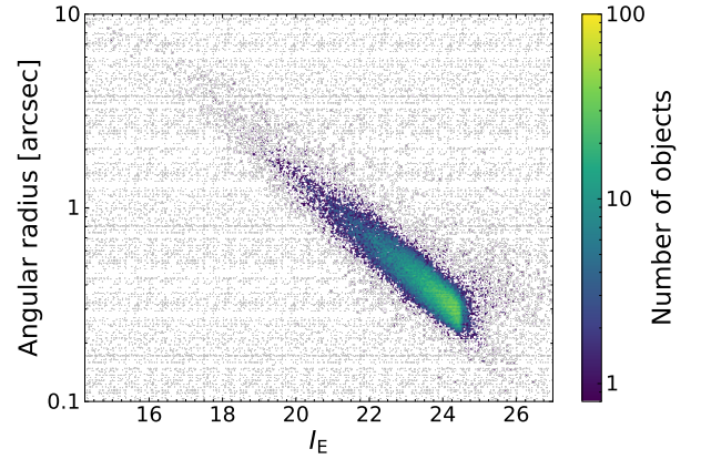
Fig. 1. Distribution of the angular radii corresponding to the isophotal areas calculated by SourceXtractor++ on all objects identified as galaxies in the ERO-Perseus field by Cuillandre et al. (2025b) versus their SExtractor’s MAG_AUTO I_E magnitude. All 38 032 modelled sources with I_E \leq 24.5 are plotted, as described in Sect. 2.3.
