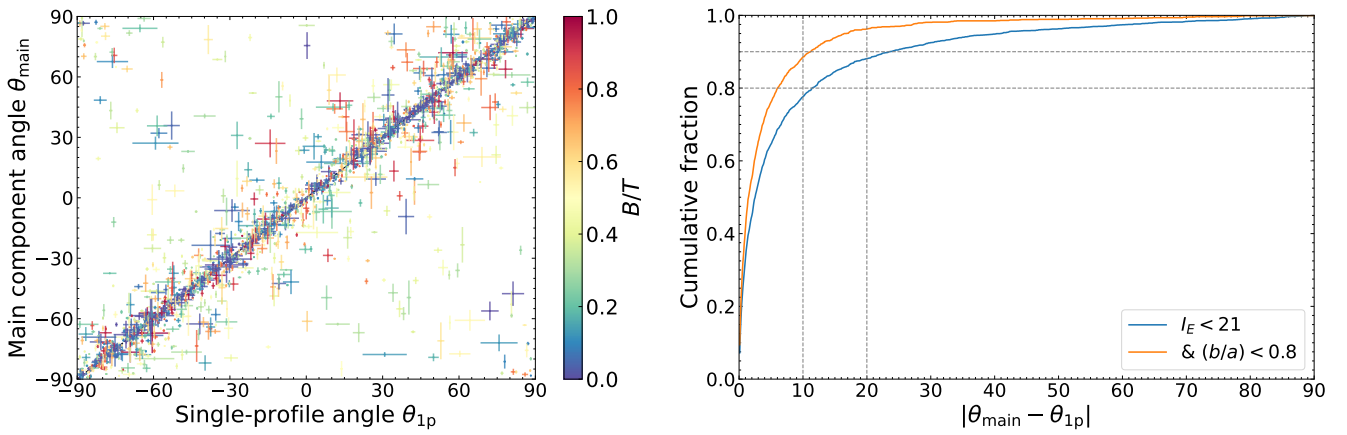
Fig. 9. Comparison between the position angle of the major axis of the single-Sérsic profile \theta_{1p} and of the dominant profile in the bulge-disc decomposition \theta_{\text{main}} (see Eq. (5)) for the 2445 galaxies with I_E \leq 21 . The left panel compares both angles, with a B/T(I_E) colour map for the points, highlighting an agreement for most of the galaxies, as well as outliers reaching up to tens of degrees of angle difference. No trend with B/T is noticeable. The right panel shows the cumulative fraction of galaxies for which the difference of \theta_{\text{main}} - \theta_{1p} is less than the value of the threshold (in degrees on the x -axis), for all galaxies with I_E \leq 21 (in blue) and limited to b/a < 0.8 for both models (in orange, corresponding to 1721 galaxies, hence 70.4% of the sample), given that the position angle of a model with elliptical symmetry can take any value when fitted to a face-on galaxy. Vertical dashed lines indicate the 10^\circ and 20^\circ thresholds, while horizontal dashed lines show the 80% and 90% fractions. The right panel confirms quantitatively the agreement between the two position angles observed in the left panel, with 89% and 96% of non-face-on galaxies having a difference in their measured angles below 10^\circ and 20^\circ , respectively.
