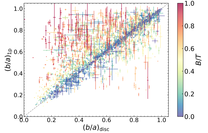
Fig. 7. Comparison of the axis ratio for the 2445 galaxies with I_E \leq 21 modelled as single-Sérsic profiles with that of the disc derived from the bulge-disc decomposition, colour-coded by the overall morphologies of galaxies, parametrised with B/T(I_E) . This graph shows agreement in the axis ratio of the single-Sérsic profile and the disc component for low B/T galaxies. The axis ratio is significantly larger for the single-Sérsic profile than for the disc component for galaxies with prominent bulges, therefore providing an underestimation of their disc inclinations.
