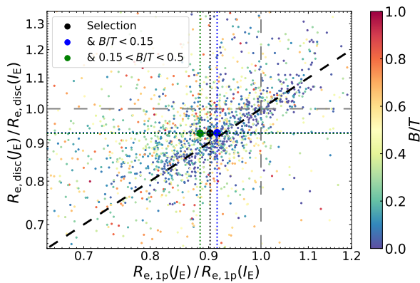
Fig. 17. Comparison between the ratio of effective radii measured in the J_{\text{E}} and I_{\text{E}} bands for the single-Sérsic profile ( x axis) and for the disc component ( y axis) of the 2047 galaxies with R_{\text{e,disc}}/R_{\text{e,bulge}} \geq 1 and R_{\text{e,disc}}/R_{\text{e,1p}} > 0.9 in the I_{\text{E}} band. The colour of the points represent the bulge-total ratio B/T in the bulge-disc decompositions. The black, blue, and green crosses correspond to the medians for the [0, 1], [0, 0.15], and [0.15, 0.5] B/T subsamples, after selecting galaxies with both R_{\text{e}} ratios in the [0.7, 1.2] interval. Both ratios, hence colour gradients, show a similar behaviour, as seen in Figs. 15 and 16, with ratios below unity indicating that redder stellar populations are more concentrated in galaxy centres. The disc and single-Sérsic ratios are similar for B/T \approx 0 but for larger bulges, the single-Sérsic ratio decreases further away from 1, whereas the disc ratio remains stable (bootstrap uncertainties are provided in the text). Because single-Sérsic profile models both the bulge and the disc, and the latter is made up of bluer stars than the former in spiral galaxies, it displays a stronger overall colour gradient in galaxies with more prominent bulges.
