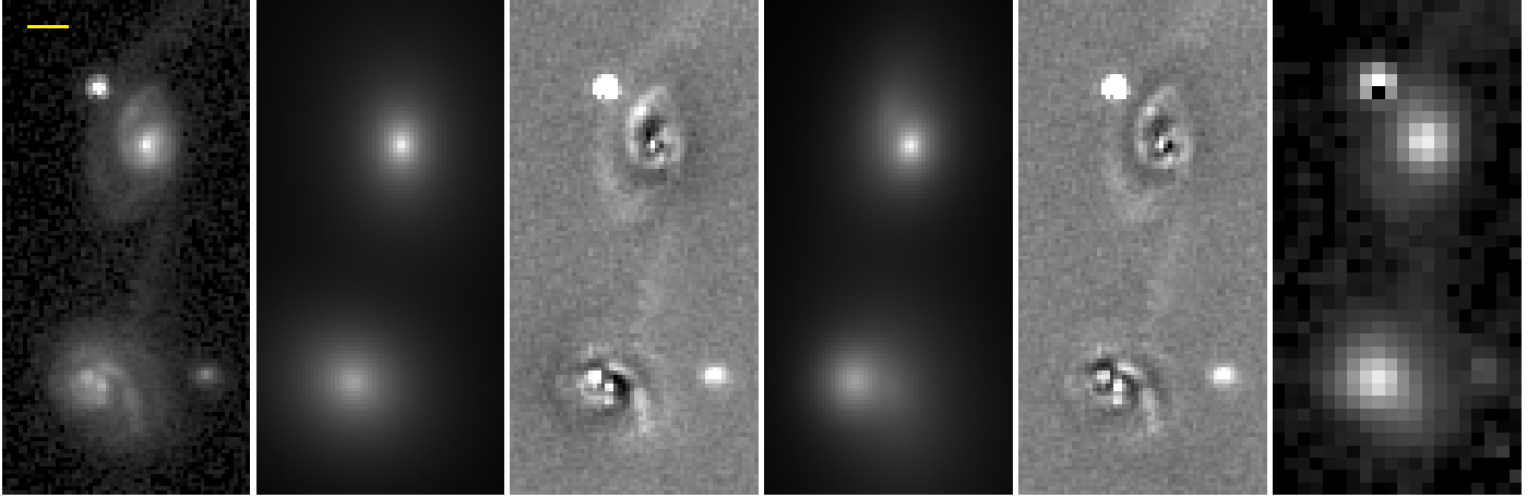
Fig. B.18. Objects 18a and b: a pair of spiral galaxies probably undergoing an interaction, since a ‘plume’ of matter appears to connect them and their discs are asymmetric, hence their being displayed together, with Object 18a at the bottom and Object 18b at the top. Although the single-Sérsic fit residuals appear similar to those from the bulge-disc decompositions, the latter models for both galaxies have a disc and bulge offset in their centring due to the disc asymmetries: in Object 18a, the disc model is positioned to the right of the bulge model, while in Object 18b, it is to the upper left. For both objects, the effective radius of the single-Sérsic fit is nearly the average of those of the bulge and the disc, which could give the false impression of two successful bulge-disc decompositions – it is the split between the disc and bulge centres that indicates that these bulges and discs are not physical. Moreover, in Object 18a, the central part of the galaxy hosts two bright spots, one of which may be a bulge and the other a bright H II region (perhaps triggered by the interaction). None of these spots in Object 18a are modelled by the bulge component, which has too low a Sérsic index ( n_B = 0.82 ). In contrast, the bulge of Object 18b is well defined but is as much underestimated in flux by the bulge model as by the single-Sérsic fit. However, the disc model being offset towards the spiral arm (to the upper-left) leads the bulge model to also include the inner disc around the bulge, yielding an overestimated B/T = 0.76 and a likely underestimated n_B = 1.97 . Lastly, for both galaxies, the single-Sérsic fit indices are similar to those of the bulge component, leaving significant residuals, comparable to those for the bulge-disc decomposition, and also caused by the disc asymmetry. The bulge-disc decomposition would be largely unconstrained with the Y_E lower angular resolution, in which the well-designed spiral arms seen in the I_E band are undetectable.
