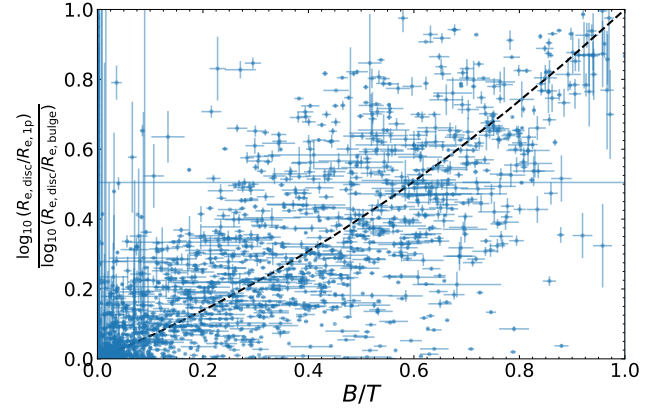
Fig. 4. Correlation between the disc-to-single Sérsic ratio of effective radii relative to the disc-to-bulge ratio of radii (in logarithmic scale) and B/T in the I_E band for the 1826 galaxies with I_E \leq 21 , verifying R_{e,bulge} < R_{e,lp} < R_{e,disc} .
