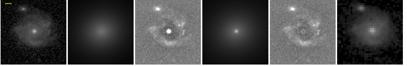
Fig. B.2. Object 2: same as for Object 1.
