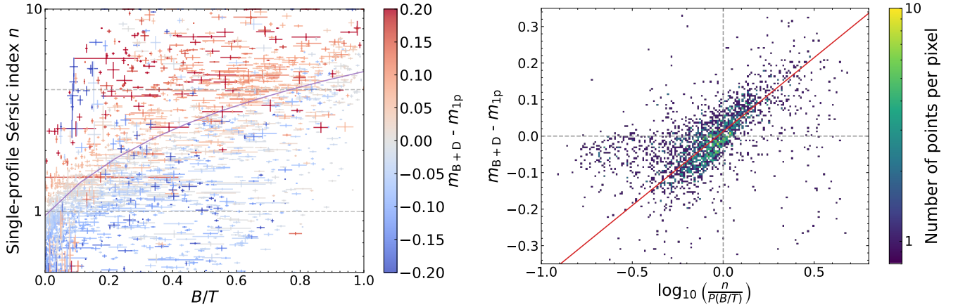
Fig. 13. Relations between the difference in the model magnitudes of both model configurations and the difference in the Sérsic index n for the single-Sérsic fit and B/T of the bulge-disc decomposition for the 2445 galaxies to I_E \leq 21 . Left: value of n as a function of B/T . The I_E magnitude difference between the two models is shown as the colour of the points. The first-degree polynomial best-fitting P(B/T) = n appears as a purple line and matches the separation between the positive and negative magnitude differences, which appear mostly above and below it, respectively. Right: magnitude difference plotted as a function of the distance between points in the left panel and the best-fit relation computed vertically and in logarithmic scale. The vertical m_{1p} - m_{\text{auto}} offset in Fig. 12 can therefore be explained as the result of a discrepancy between the measured n and B/T , with less flux within the bulge-disc decomposition than the single-Sérsic model of a galaxy since its n is larger than what should be expected from its B/T through their fitted linear relation (and inversely). A difference in model photometry is therefore correlated to a discrepancy between the two parameters, which, in each configuration, better describe the overall galaxy morphology.
