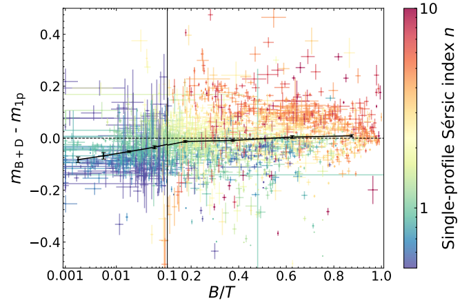
Fig. 12. Difference between the model magnitudes obtained from the bulge-disc decomposition and the single-Sérsic fit as a function of B/T for the 2445 galaxies with I_E \leq 21 . The solid black line separates two areas of the graph, with logarithmic and linear scales to the left and to the right, respectively, whereas black dots correspond to median and bootstrap errors in bins of B/T . For small B/T , the bulge-disc decomposition leads on average to brighter magnitudes, but this median offset vanishes for more prominent bulges ( B/T \gtrsim 0.2 ). A strong vertical colour gradient appears at all B/T , with higher (smaller) n corresponding to more (less) flux in the single-Sérsic model than in the bulge-disc one.
