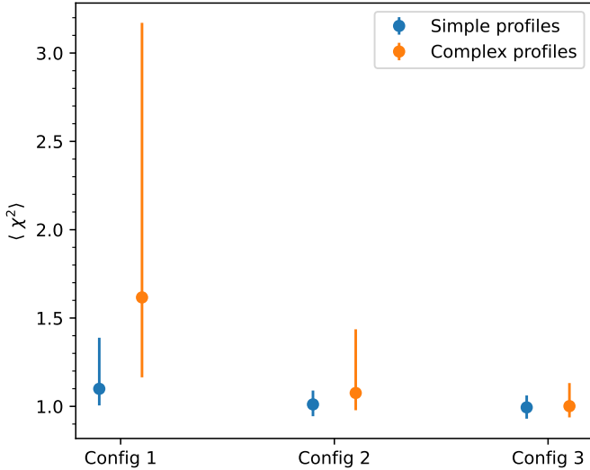
Fig. 7. Quality of the inversions for the different node configurations of increasing complexity (see Table 1). The filled circles are the average \chi^2 (Eq. (4)) calculated for profiles whose total dimensionality is smaller (simple) or larger (complex) than 80 (see binary mask in Fig. 4). The error bars show the 16th and 84th percentiles of each distribution.
