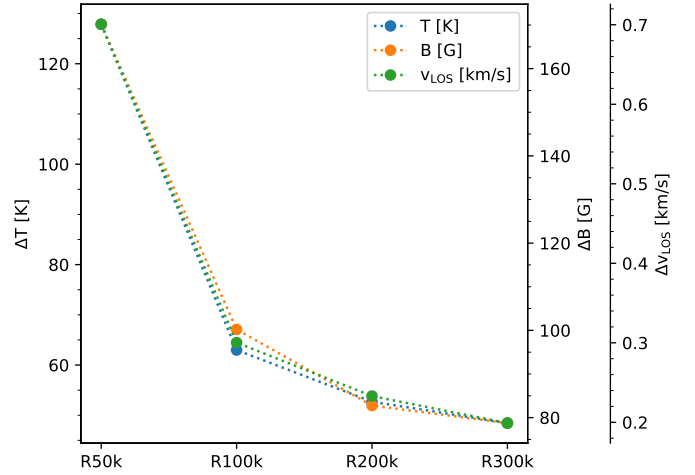
Fig. 12. Average error in the temperature, magnetic field strength, and line-of-sight velocity for the most realistic case (degraded, noisy, and resampled) using configuration 2 for different spectral resolutions.
