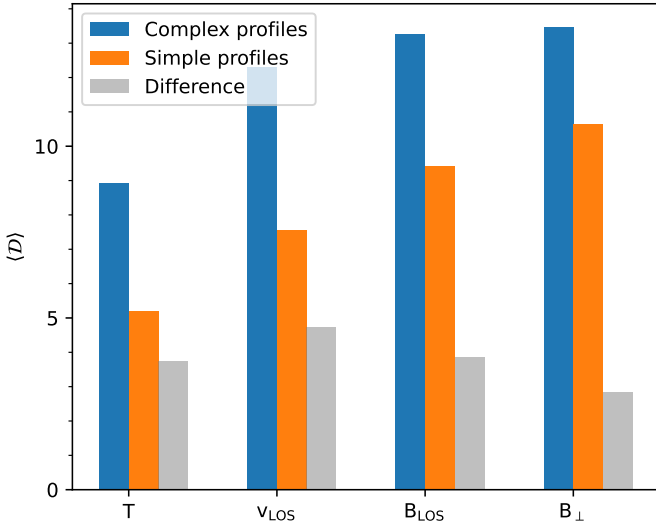
Fig. 10. Average dimensionality of the physical quantities in the simulation calculated from stratifications belonging to simple and complex profiles. The gray bars show the difference between the two.
