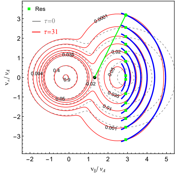
Fig. 2. Contours of proton VD for run 4 at \tau = 0 (dashed gray) and at \tau = 31 (solid red), when the forward-half of VD is shaped by the kinetic shells (blue) that were found relevant for the hammerhead populations reported by PSP (Verniero et al. 2022). The diffusion contours v_\perp(v_\parallel) were computed by linking the proton coordinates (v_\parallel, v_\perp) (green squares) with the resonant wave frame (v_{\phi,r}/v_A = 1.3, 0.0) (black dot) and \tilde{k}_r = 0.60 . The slope of these lines, such as the green line, is v_\perp/[v_\parallel - v_\phi] , with v_\parallel and v_\perp calculated using Eqs. (14) and (15) in Isenberg & Lee (1996).
