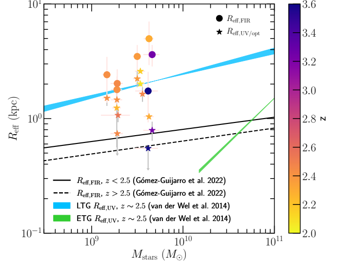
Fig. 8. Far-infrared dust continuum effective radius (filled circles) and rest-frame UV/optical effective radius (filled stars) as a function of the stellar mass of our galaxies, colour-coded by redshift. All our galaxies have systematically higher R_{\text{eff,FIR}} than R_{\text{eff,UV/opt}} . As a result, R_{\text{eff,FIR}} of our galaxies strongly deviate from the R_{\text{eff,FIR}}-M_{\text{stars}} relations of Gómez-Guijarro et al. (2022) at z < 2.5 and z > 2.5 , shown by the solid and dashed black lines, respectively, as they are more extended. On the other hand, their R_{\text{eff,UV/opt}} agree with the R_{\text{eff,UV}}-M_{\text{stars}} relation (blue shaded area) derived for LTG at z \sim 2.5 by van der Wel et al. (2014). The green shaded area corresponds to the R_{\text{eff,UV}}-M_{\text{stars}} relation of z \sim 2.5 early-type galaxies (ETG; van der Wel et al. 2014).
