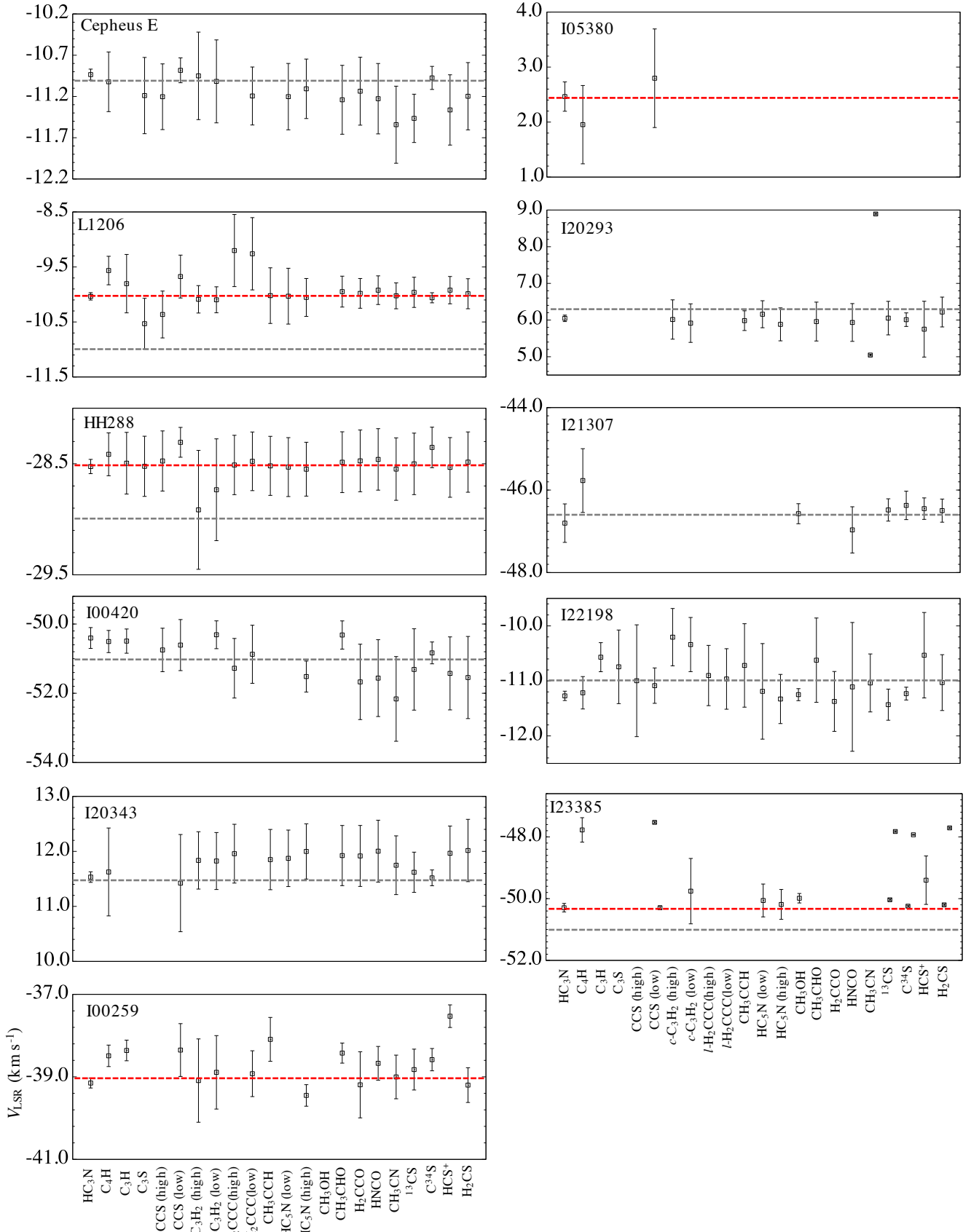
Fig. A.2. Comparison of the centroid velocity ( V_{\text{LSR}} ) obtained via the MCMC analyses. The error bars do not include the velocity resolution of spectra ( \approx 0.3 km s ^{-1} ). The dashed gray horizontal lines indicate the systemic velocity of the source (Table 1). The dashed red horizontal lines indicate the systemic velocity updated or reported based on our results.
