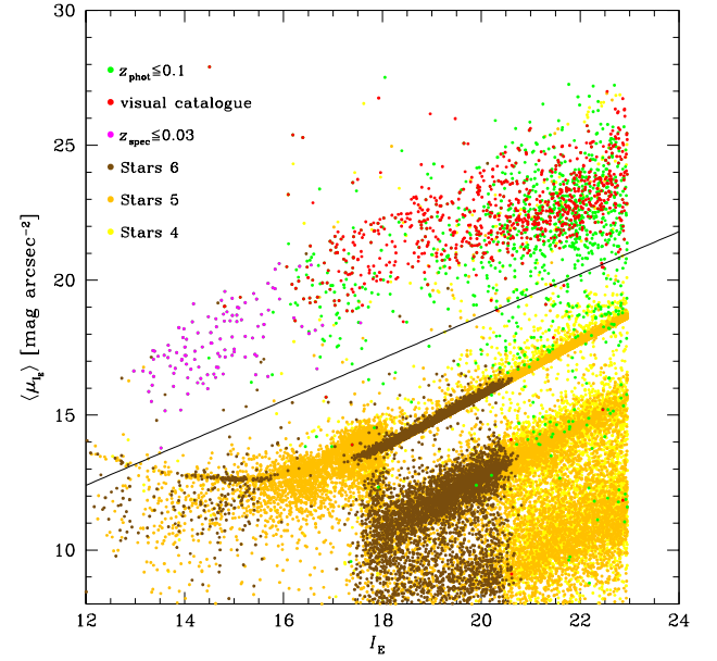
Fig. 20. Relation between the mean versus model effective surface brightness and the total magnitude for all sources in the full SourceExtractor catalogue with I_E \leq 22.96 . Brown, orange, and yellow dots are for targets classified as stars consistently by six, five, and four independent criteria, respectively. Green dots are for galaxies with photometric redshifts from Phosphoros z_{\text{phot}} \leq 0.1 , red dots for optically identified cluster members, and magenta dots for spectroscopically confirmed cluster members ( z_{\text{spec}} \leq 0.03 ). The black solid line ( \langle \mu_E \rangle = 0.783 I_E + 3 \text{ mag arcsec}^{-2} ) delimits the region where most (13/899, 1.4%) of the spectroscopically and visually identified members are located.
