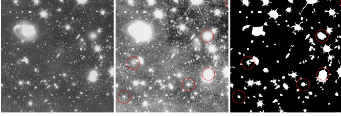
Fig. 14. Left: Section of the original VIS image (900 pixels \times 900 pixels, 90'' on the side) displaying standard features, specifically extended cluster galaxies, stars, background galaxies, and optical ghosts near bright stars, which appear as faint round structures. Middle: Ring-filtered version enhancing extended sources and removing compact ones. The red circles (10'' in diameter) mark the dwarfs from our catalogue of members. Right: SourceExtractor segmentation map confirming detection of all dwarfs and maintaining a low count of other detected sources.
