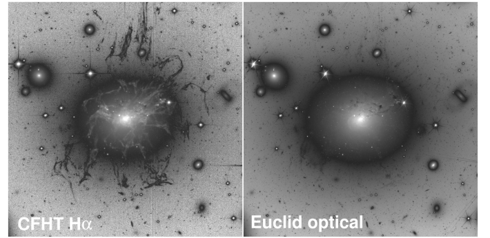
Fig. 5. Left: Image of H \alpha + [N II] emission from the galaxy NGC 1275 by CFHT. The filamentary structures show the cooling flow gas (e.g. Conselice et al. 2001). Right: Euclid I_E image. The FoV per panel is 4' by 4'.
