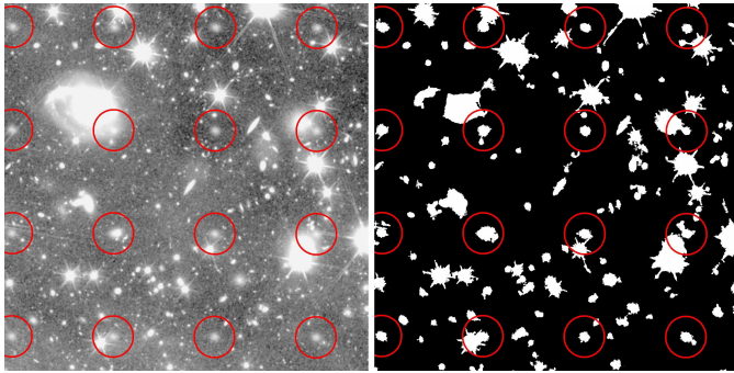
Fig. 16. Injection of simulated galaxies. Left: Simulated I_E = 22.4 dwarf galaxy with specific physical parameters (Sérsic index = 0.61, I_e = 0.49 ADU per pixel, R_e = 18.10 pixels, ellipticity = 0.14, and position angle = 72^\circ ) injected into a 250 \text{ pixel} \times 250 \text{ pixel} grid (marked by red circles). Right: SourceExtractor segmentation map showing successful recovery of most injected sources. This example clearly demonstrates how completeness is compromised by crowding from nearby stars and galaxies. The image area is the same as in Fig. 14.
