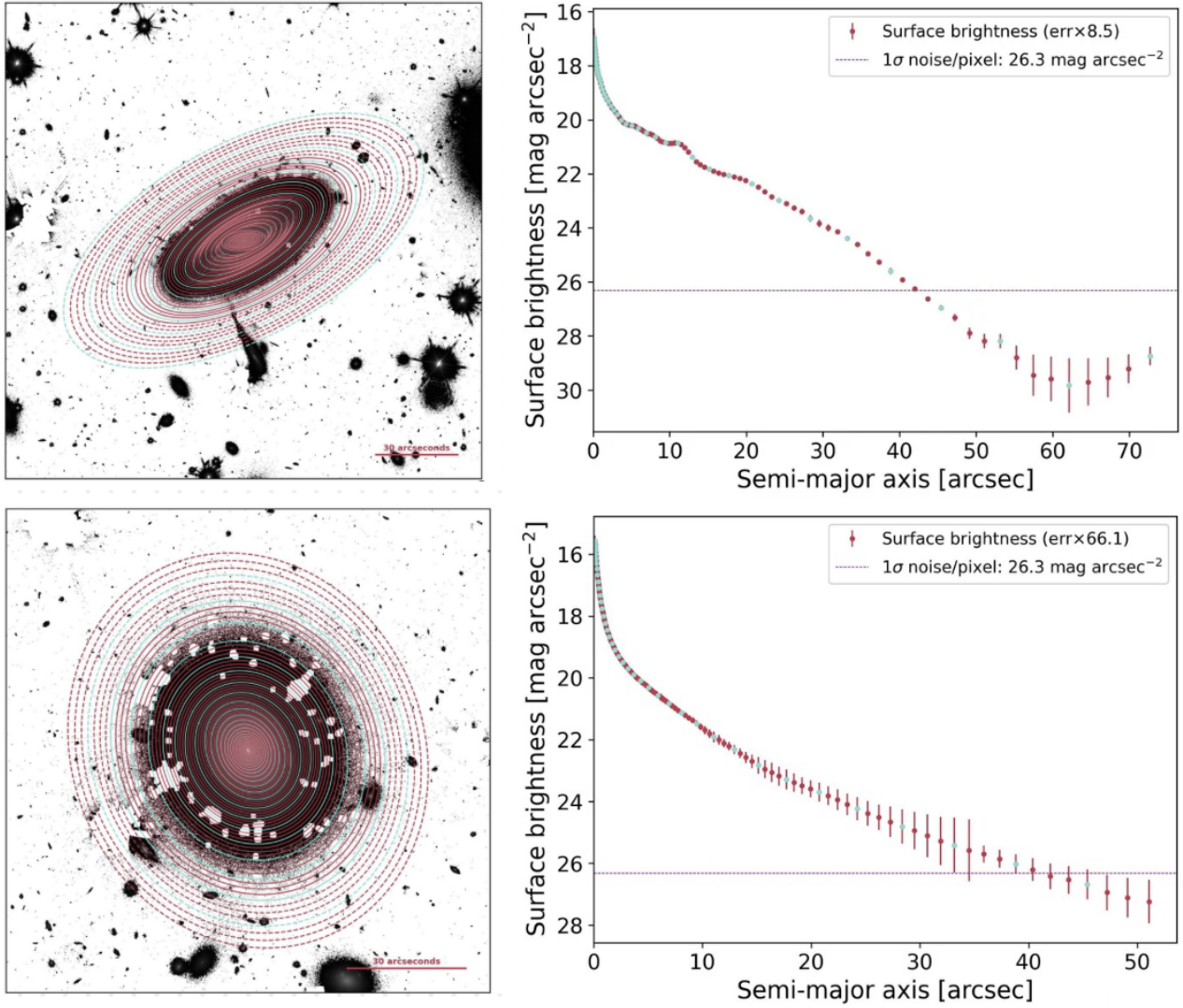
Fig. B.1: Examples of AutoProf radial profile extraction on VIS data to derive photometric and morphological properties. Top left : UGC 02665 isophote fitting on an 2000\text{ pixel} \times 2000\text{ pixel} pixel cutout ( 200'' \times 200'' , red angular scale on the image: 30'' ). Top right : Radial surface brightness profile for UGC 02665, showing a dip at r = 60'' due to overlap with neighbours, marking the photometry's limit. Bottom left : WISEAJ031858.26+414208.7 isophote fitting on a 2000\text{ pixel} \times 2000\text{ pixel} pixel cutout ( 200'' \times 200'' , red angular scale on the image: 30'' ). Bottom right : Radial surface brightness profile for NGC 1281, reaching down to 30.1\text{ mag arcsec}^{-2} at r = 100'' despite the proximity of a bright star. Cyan and red points on the radial profiles refer to the colours of isophotes in the associated AutoProf visual, which help guide the eye when comparing plots.
