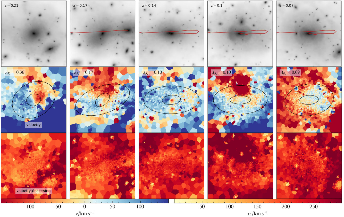
Fig. 7. Evolution of the first example galaxy from Fig. 1. The shells develop after a massive radial merger event, which also causes the value of \lambda_{R_c} to sharply drop and converts the galaxy into a slow rotator (where \lambda_{R_c} is measured from the edge-on projection). Top: mock images of the stellar component from a projection in which the shells are especially clearly visible. The red lines trace the orbit of the infalling galaxy until the respective point in time. Middle: velocity maps. The circles indicate the ellipses at one and three half-mass radii. Bottom: velocity dispersion maps.
