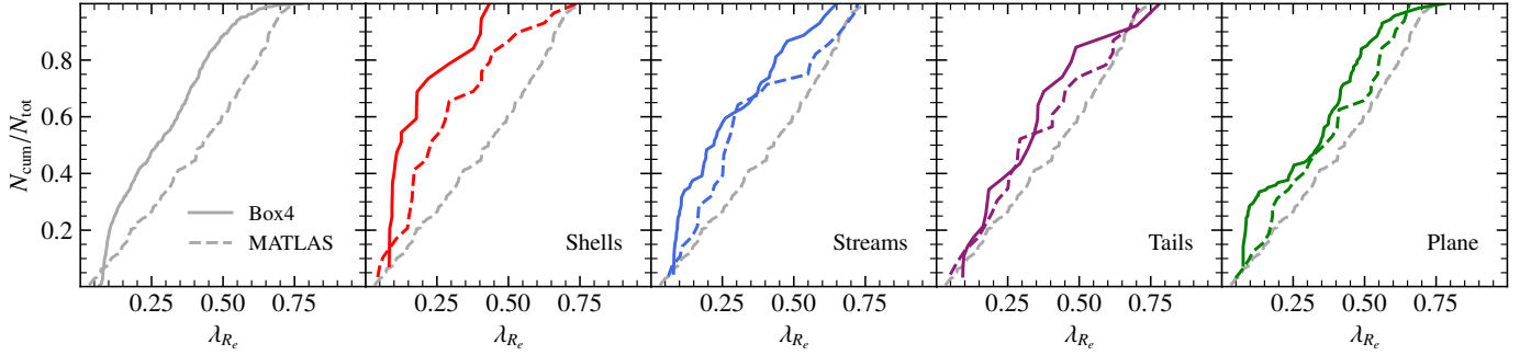
Fig. 6. Cumulative histograms of \lambda_{R_c} for the galaxies in the MATLAS survey (dashed lines) and in Magneticum Box4 (uhr) (solid lines). Only the ETGs and intermediate-type galaxies were considered for the simulated sample. The first plot shows the difference in the distributions between observations and simulations. The cumulative histograms of the simulated galaxies in the other four panels were adapted to match the parent distribution of MATLAS to be directly comparable to the distributions of the MATLAS survey. The colored lines lying above the dashed gray line (the overall distribution of the MATLAS survey) indicate an increased presence of the respective tidal feature or satellite plane for galaxies with lower rotational support compared to those with higher rotational support. The measurements of shells, streams, and tails of MATLAS galaxies are taken from Bílek et al. (2020) , and the measurements of the planes are taken from Heesters et al. (2021) .
