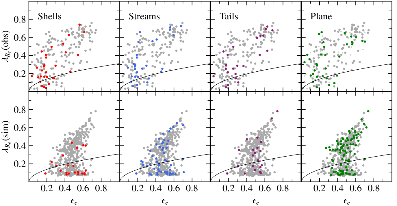
Fig. 5. Galaxies classified as having tidal features or a satellite plane in the \lambda_{R_e}-\epsilon_e plane in the MATLAS survey (top row) and in Magneticum Box4 (bottom row). Only the ETGs and intermediate-type galaxies are shown for the simulated sample. The colored data points represent galaxies with the respective feature. The large gray dots were classified as lacking the respective feature, and small gray dots were not classified (only the case for the observed satellite planes). The values of \lambda_{R_e} and \epsilon_e were determined at one effective radius for the observations and at one half-mass radius for the simulations. For the simulations, they were determined in the edge-on projection. The solid black lines indicate the border between fast and slow rotators (Emsellem et al. 2011), with fast rotators lying above the border. The measurements of shells, streams, and tails of MATLAS galaxies are taken from Bílek et al. (2020) and the measurements of the planes are taken from Heesters et al. (2021).
