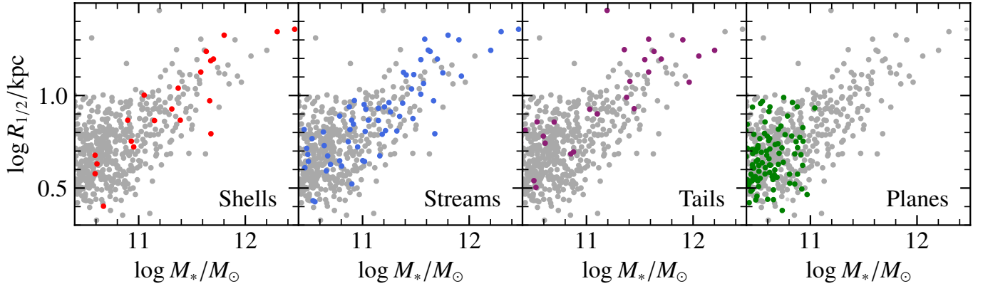
Fig. 2. Mass-size relation of the Magneticum galaxy sample. Galaxies are classified as having tidal features or satellite planes in color.
