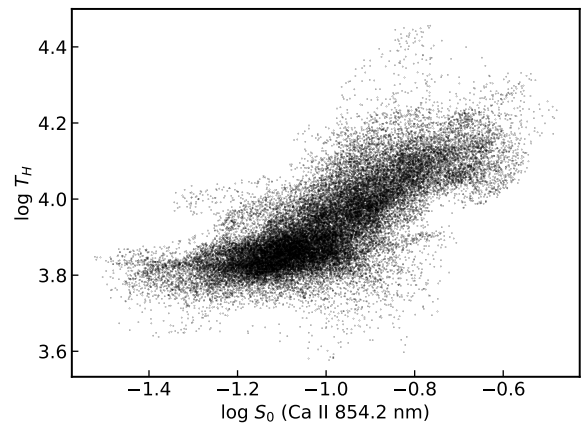
Fig. 8. Scatter plot of T_H vs. the Ca II line S_0 .
