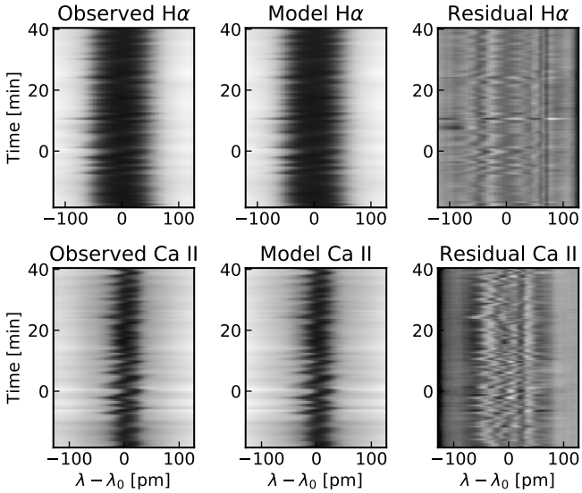
Fig. 9. Wavelength-time maps of the H\alpha and Ca II intensity stacked over time – observation ( left ) and model ( middle ), and maps of residual intensity normalized by the continuum intensity ( right ). The grey scale of the normalized residual intensity spans from -0.03 to 0.03 .
