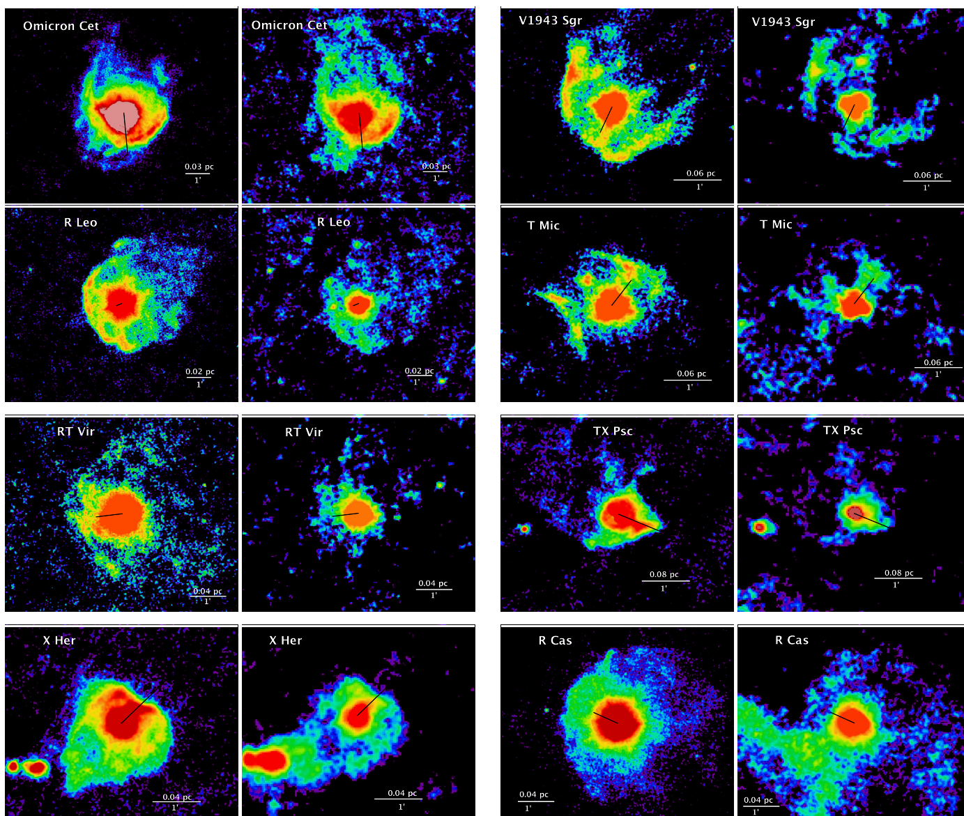
Fig. 1. continued. Interaction type “fermata” (Class I). PACS 70 \mu\text{m} (left) and 160 \mu\text{m} (right). o Cet, R Leo, RT Vir, and X Her reveal RT and/or KH instabilities. For o Cet see also Mayer et al. (2011). The sources visible eastward of X Her are background galaxies (see also Jorissen et al. 2011).
