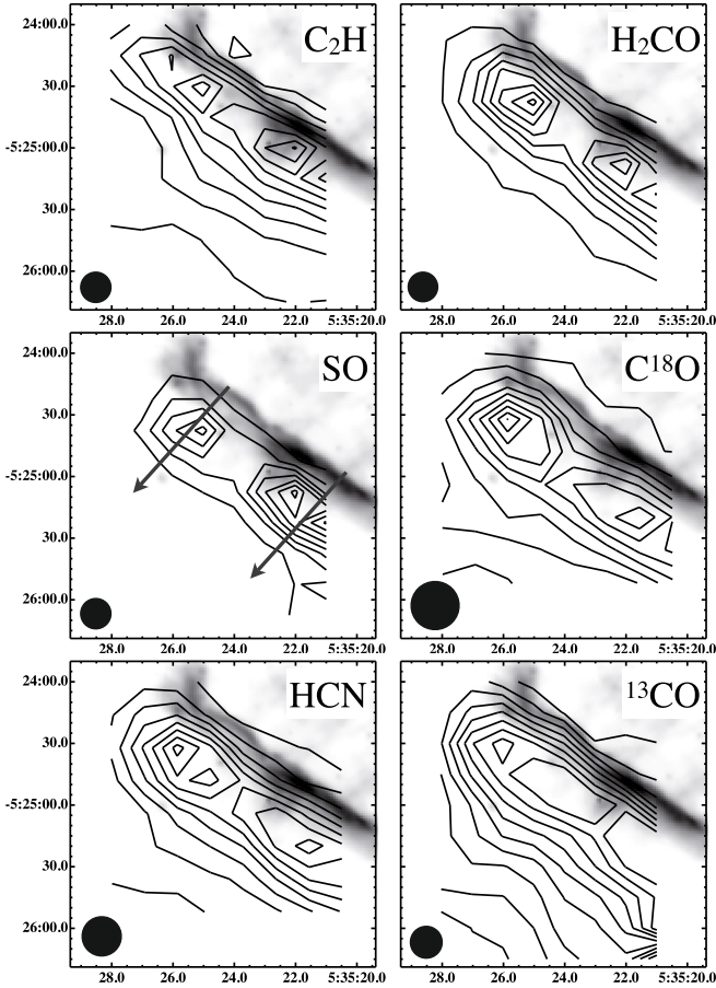
Fig. 1. Images of molecular emission, observed with the JCMT toward the Orion Bar of the species and transitions listed in Table 1. Line intensities are integrated over 5\text{--}8\text{ km s}^{-1} , depending on the line width. The \text{C}_2\text{H} transition shown here is the 4_{9/2}\text{--}3_{7/2} transition; the other transition shows a similar spatial distribution. Contour levels are drawn at 10, 20, ..., 90% of the maximum integrated intensity for every map: 13.3\text{ K km s}^{-1} for \text{C}_2\text{H} , 8.7 for \text{H}_2\text{CO} , 7.7 for \text{SO} , 19.9 for \text{C}^{18}\text{O} , 70.5 for \text{HCN} , and 276.8 for ^{13}\text{CO} . Note that the measured maximum \int T_{\text{mb}} dv values across the northeast slices (Table 1) are not the same as the highest value across the entire map. The grayscale background image shows Spitzer Space Telescope 8\text{ }\mu\text{m} continuum emission. The filled circle in each frame indicates the beam size at the relevant frequency. Axes are annotated with right ascension and declination (J2000).
