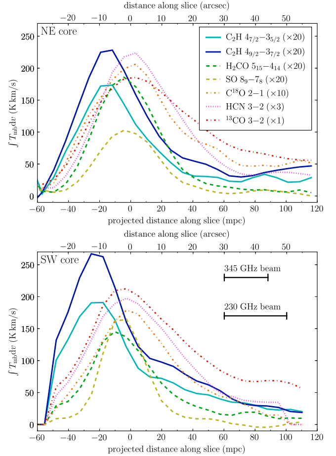
Fig. 2. Profiles of molecular emission along slices perpendicular to the ionization front at position angle 225^{\circ} (see arrows in Fig. 1): ( top panel ) through the northeast core; ( bottom panel ) through the southwest core. The zero point of the distance scale is placed at the \text{C}^{18}\text{O} peak position: ( \text{RA} = 5^{\text{h}}35^{\text{m}}25^{\text{s}}.4 , \delta = -5^{\circ}24'37'' ) for the northeast slice and ( \text{RA} = 5^{\text{h}}35^{\text{m}}21^{\text{s}}.6 , \delta = -5^{\circ}25'19'' ) for the southwest slice.
