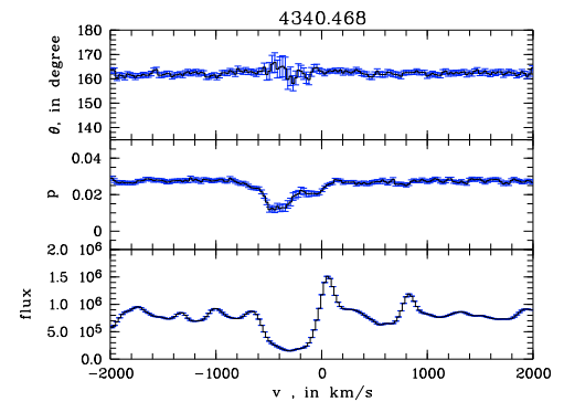
Fig. 3. Spectropolarimetry of Z CMa in H_\gamma .
