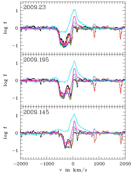
Fig. 4. Logarithmic spectral shape of the Balmer lines H_\alpha to H_9 .
