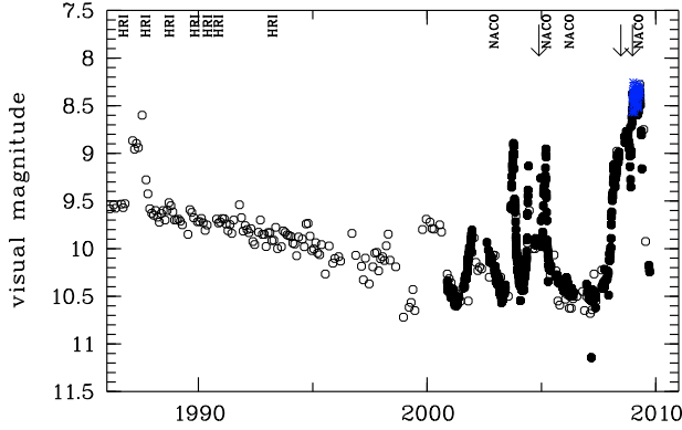
Fig. 1. Light curve of Z CMa over the last decades. Open symbols denote the observations from the American Associations of Variable Stars Observers (AAVSO). The filled symbols correspond largely to the ASAS data and during the peak of the light curve to our measurements (blue asterisks). Epochs of NACO observations, the high resolution images as summarized by Thiébaud et al. (1995) and the epoch of spectropolarimetric observations (arrows) are indicated on the top.
