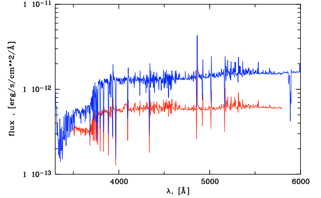
Fig. 2. Spectrophotometric flux of Z CMa in 2004 (lower spectrum) and 2008 (upper spectrum).
