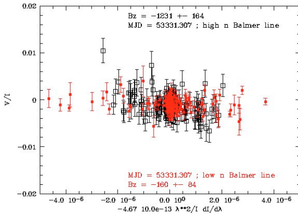
Fig. 6. Magnetic field measurements using the data obtained in November 2004. The longitudinal magnetic field is derived following the equation V/I = -g_{\text{eff}} C_z \lambda^2 \frac{1}{I} \frac{dI}{d\lambda} \langle B_z \rangle from the slope of the linear fit through the data points (see Bagnulo et al. 2002). Large open and small filled symbols are obtained from the high number and low number Balmer lines, respectively.
