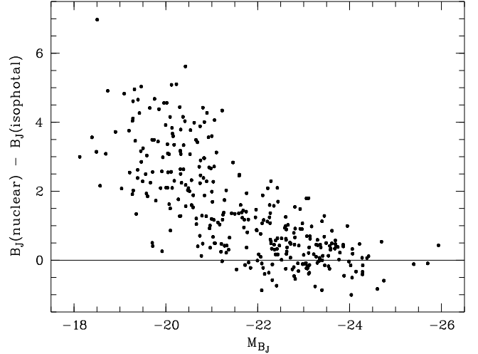
Fig. 5. Difference between “isophotal DSS” and “nuclear” magnitudes, plotted against absolute nuclear magnitude M_{B_j} .
