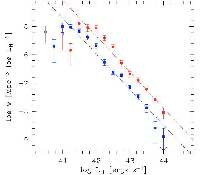
Fig. 8. Binned emission line AGN luminosity functions, for H\alpha (red filled circles) and H\beta (blue squares). Open symbols indicate incompletely filled bins. The dashed lines show the best fit single power law to the H\alpha and H\beta data, respectively.
