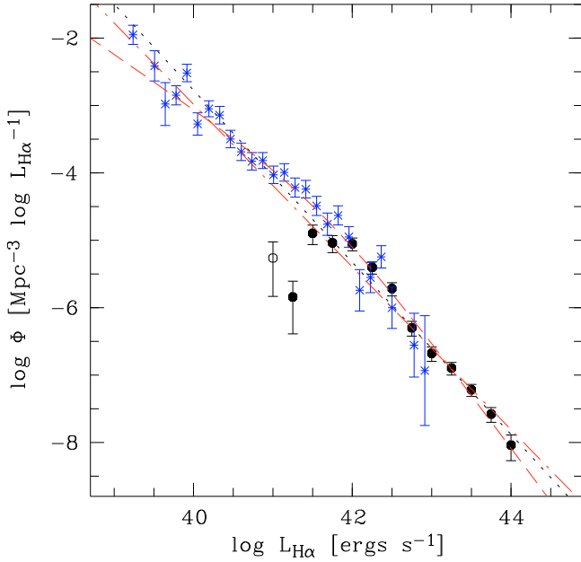
Fig. 9. Comparison of the H\alpha luminosity function derived in this work (black points), with the work of Hao et al. (2005a) (blue asterisks). The black dotted line gives the best fit single power law to our H\alpha luminosity function. The red dashed dotted line gives the best fit power law to the combined data set, whereas the red dashed line gives the best fit double power law.
