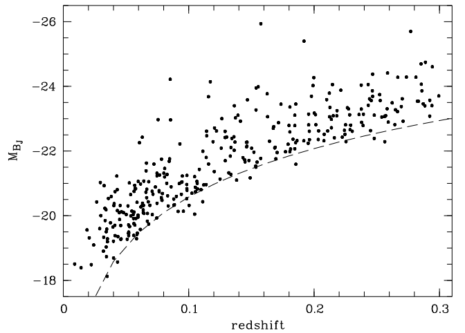
Fig. 2. Redshift against absolute magnitude M_{B_J} . The dashed line indicates a constant apparent magnitude of 17.5 mag, approximately the flux limit of the HES.
