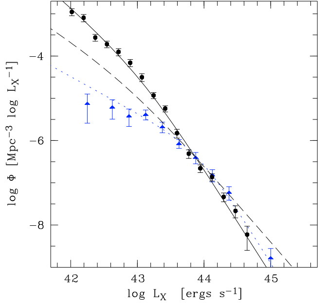
Fig. 11. Comparison of the soft X-ray LF of type 1 AGN by Hasinger et al. (2005) with the prediction based on the optical local AGNLF. The filled blue triangles show the binned X-ray (0.5–2 keV) LF within z = 0.015 – 0.2 , corrected to z = 0 . The blue dotted line shows the LDDE model of Hasinger et al. (2005) for z = 0 . The filled black circles and the solid line show the binned data and the double power law fit to the optical HES+SDSS LF, converted to soft X-rays using a luminosity dependent correction. The dashed line shows the same double power law fit, but converted to soft X-rays using a constant correction.
