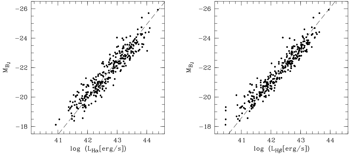
Fig. 6. Relation between absolute magnitudes in the B_J band and line luminosities ( left : H\alpha , right : H\beta ). A fixed-slope relation M_{B_J} \propto -2.5 \log L is shown as a dashed line in each panel, for illustration purposes only.
