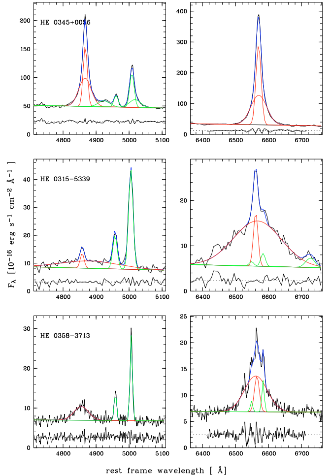
Fig. 3. Examples of fits to the spectra, illustrating the quality of the spectroscopic data. The line complex of H\beta is shown on the left side, the corresponding complex around H\alpha is shown on the right side. The data are represented by black lines, the multi-component Gaussian fits to the Balmer lines are shown in red, other lines are shown green, and the combined model is overplotted in blue. Each panel also shows the fit residuals at the bottom.
