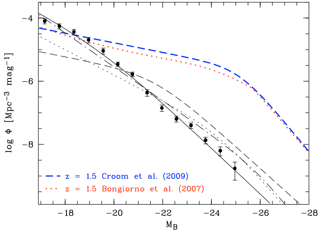
Fig. 12. Shape evolution and “downsizing” of the AGNLF between z = 1.5 and z = 0 . Filled circles and solid line denote our combined HES+SDSS AGNLF at z = 0 . The blue dashed and red dotted lines show the best fit model to the data of the z = 1.5 AGNLF of the 2SLAQ+SDSS (Croom et al. 2009b) and the VVDS+SDSS (Bongiorno et al. 2007), respectively. The thin black dashed, dashed-dotted and dotted lines show the z = 0 extrapolations of the LEDE model and the LDDE model by Croom et al. (2009b) and the LDDE model by Bongiorno et al. (2007), respectively.
