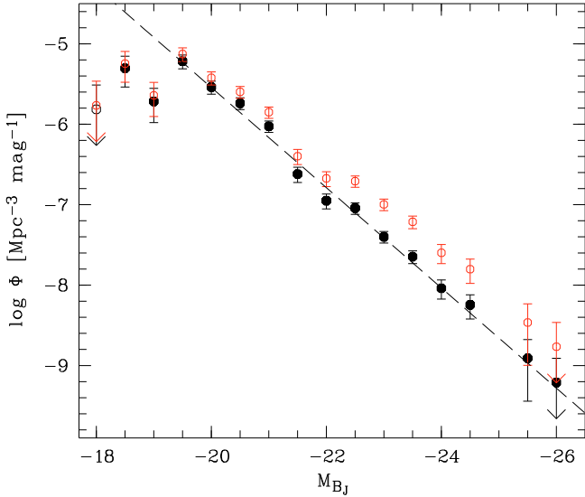
Fig. 7. The differential broad band quasar luminosity function of the HES for 0.01 \leq z \leq 0.3 . The error bars are based on Poisson statistics. The arrow indicates a bin with only a single object. The black filled symbols show the luminosity function corrected for evolution using a simple PDE model; red open symbols show the LF not corrected for evolution. The dashed line shows a single power law fit to the data.
