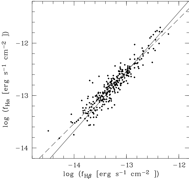
Fig. 4. Correlation between the fluxes f(\text{H}\beta) and f(\text{H}\alpha) . The solid line shows the regression result using the FITEXY method. The dashed line shows the best fit line with slope of unity.
