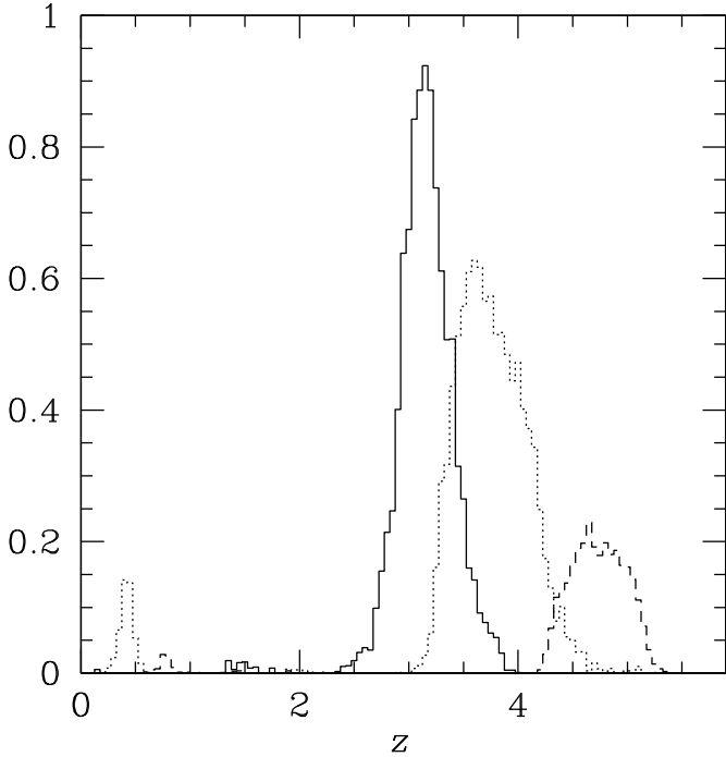
Fig. 1. Simulated redshift distributions of the three dropout samples ( u -dropouts: solid , g -dropouts: dotted , r -dropouts: dashed ; arbitrarily normalised but with correct relative fractions). The simulations are based on templates from the library of Bruzual & Charlot (1993). See Hildebrandt et al. (2009) for a detailed description of the simulations.
