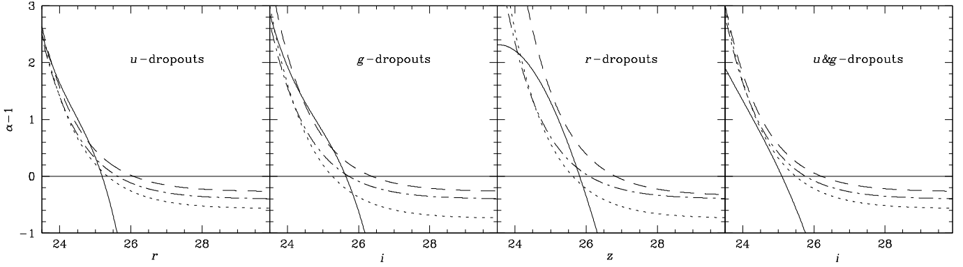
Fig. 3. Adopted values of \alpha - 1 as a function of LBG magnitude for the four background samples. The dotted, dashed, and dash-dotted lines correspond to the slopes of the LFs of Sawicki & Thompson (2006), Bouwens et al. (2007), and Steidel et al. (1999), respectively, while the solid line corresponds to the slope of the polynomial fitted to the number counts of Fig. 2.
