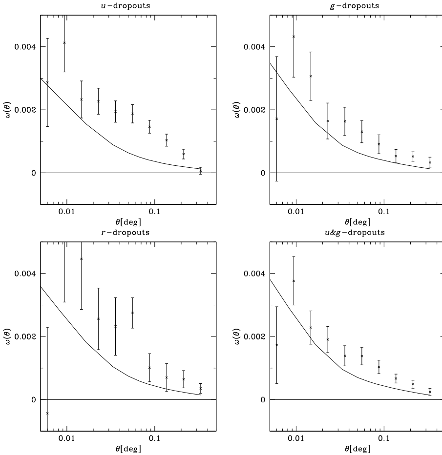
Fig. 5. Optimally weighted cross-correlation function between the complete dropout samples and the different foreground galaxy samples. The solid line correspond to the predictions based on the LF slopes of Sawicki & Thompson (2006) .
