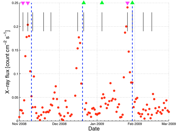
Fig. 1. X-ray lightcurve (Swift/BAT, 15–150 keV) of BP Cru in the period of our observing campaign (red dots). Vertical black lines indicate the epochs of our radio observations, and the dashed blue lines the periastron passages. Green triangles peak up indicate a positive spectral index, magenta triangles peak down indicate negative spectral index.
