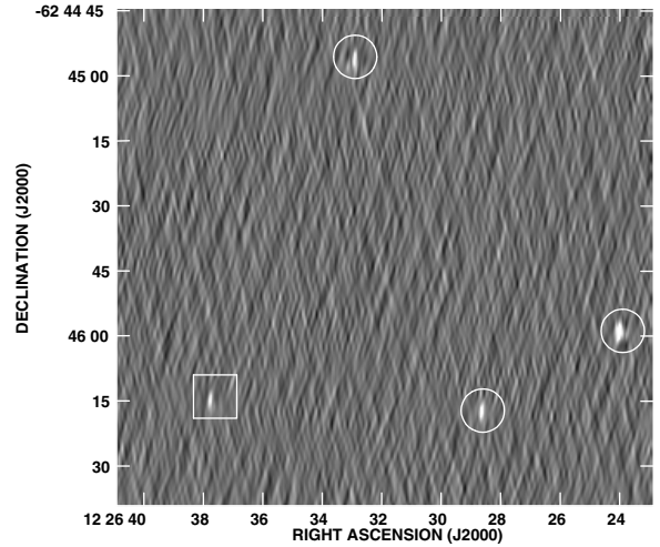
Fig. 2. Stokes I maps of the data taken in epoch 8, at 8.6 GHz. The beam size for this epoch was 3.4 \times 0.7 arcsec. The box indicates BP Cru, the circles indicate sources A (to the right), B (top in the figure) and C (lowest in the figure) as in Table 4.
