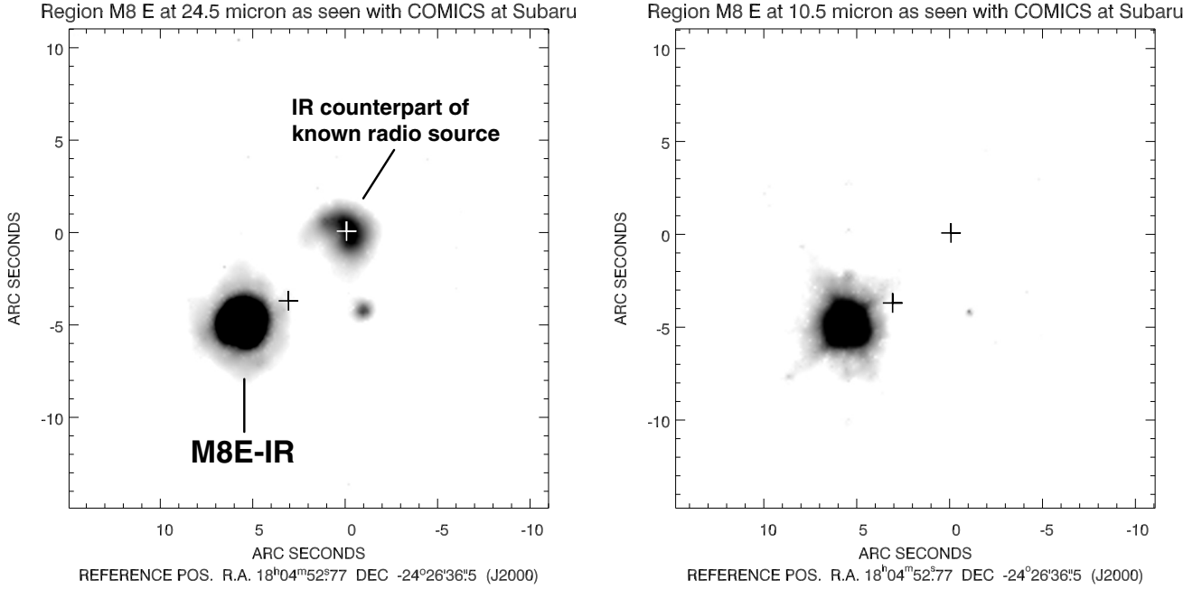
Fig. 1. Left: Q -band image of the M8E region at 24.5\ \mu\text{m} with COMICS/Subaru. The two previously known objects are annotated. The black plus indicates the position of a 44 GHz methanol maser according to Val'tts (1999). The white plus marks the position of the cm continuum source (Molinari et al. 1998). Right: N -band image of the M8E region at 10.5\ \mu\text{m} with COMICS/Subaru. The two plus signs mark the same objects as in the left image. The IR counterpart of the cm source is not detected, while the third IR source is faintly visible.
