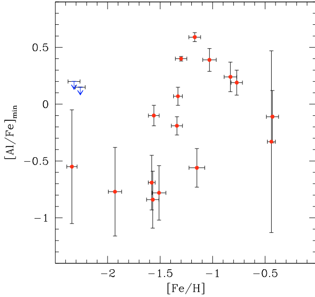
Fig. 12. [\text{Al}/\text{Fe}]_{\text{min}} versus [\text{Fe}/\text{H}] for the 19 GCs; the two upper limits are for NGC 4590 and NGC 7078.
