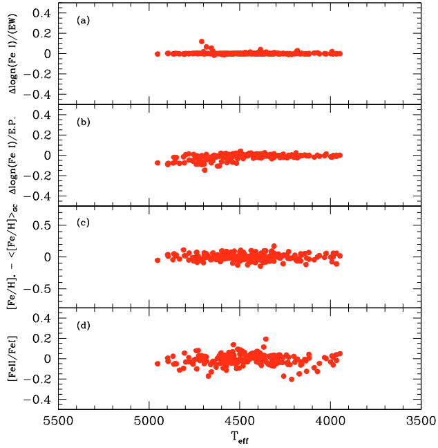
Fig. 1. A graphical summary for the analysis of iron abundances in the 202 red giant stars with UVES spectra in the 17 GCs analysed here. a): slope of the relation between expected line strength and Fe I abundances used to derive the v_t values for each individual stars. b) slope of the relation between Fe I abundances and excitation potential E.P. for each star. c): the average [\text{Fe}/\text{H}] value for each cluster is subtracted from the metallicity of each star in the cluster, and the differences are shown. d): differences in iron abundances from Fe I and Fe II lines. All quantities are plotted as a function of the effective temperature.
