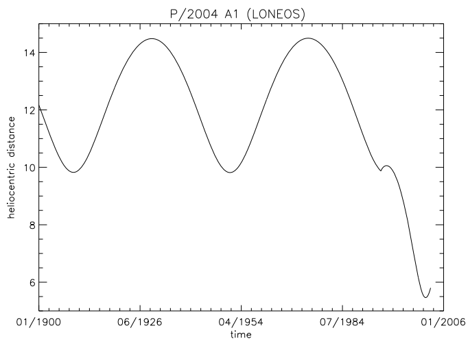
Fig. 2. The effect of Saturn's close encounter on the orbit of P/2004 A1 LONEOS: evolution of heliocentric distance from 1900 to 2006.
