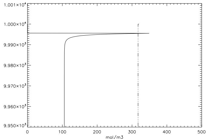
Fig. 5. Case 1 – Density profile at the end of the orbit 2 (see Table 6), at the latitude of the equator. CO (continuous line) and \text{CO}_2 (dashed line) are shown. The surface is at 10 km of the radius. The first meters close to surface are depleted in CO.
