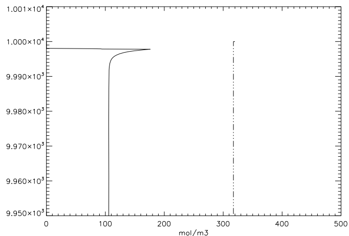
Fig. 6. Case 1 – Density profile at the end of the orbit 2 (see Table 6), at the latitude of 85^\circ . CO (continuous line) and \text{CO}_2 (dashed line) are shown. The surface is at 10 km of the radius. CO ice can be found very close to the surface.
