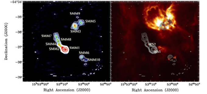
Fig. 2. Left: the image and contours represents the filtered P-ArTéMiS 450- \mu\text{m} emission where the emission over an area larger than 24'' has been filtered. The contours are the 450- \mu\text{m} emission at levels of 2, 4, 6, 8, 12, 16, 40, and 75% of the 101 \text{Jy beam}^{-1} peak flux. The rms is about 0.4 \text{Jy beam}^{-1} on the map. Right: Zoomed view of the IRAC 8- \mu\text{m} emission image. Contours represent the filtered P-ArTéMiS 450- \mu\text{m} emission.
