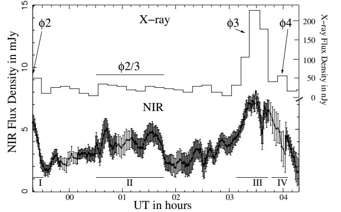
Fig. 1. The X-ray and NIR 2.2 \mu\text{m} light curves obtained on July 07, 2004 (Eckart et al. 2006a). Here we plot the data with a UT time axis and separate flux density axes for the NIR (left) and X-ray (right) data. In addition to the flare nomenclature introduced in Eckart et al. (2006a) we labeled the section of the X-ray light curve that corresponds to the NIR feature II as \phi 2/3 as it is located between \phi 2 and \phi 3 .
