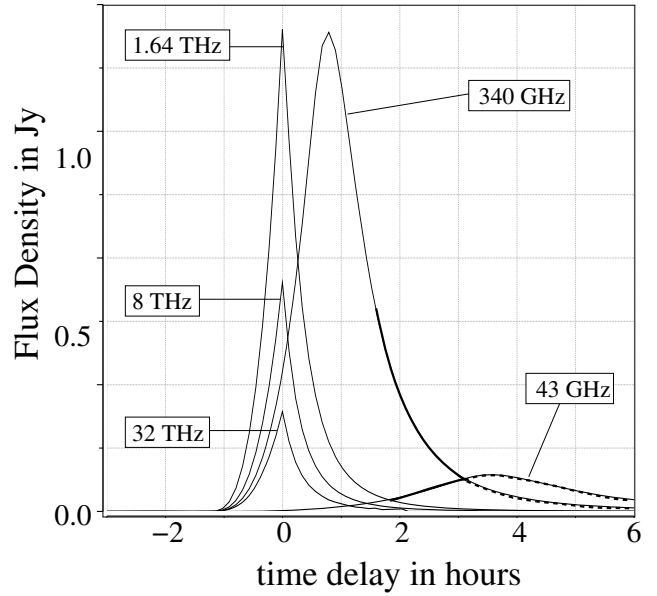
Fig. 5. The adiabatic expansion of a single source component with a peak flux density at 1.64 THz of 10 Jy, start time at 0 hours, and constant expansion velocity of 0.08 c . The 1.64 THz, 8 THz and 32 THz light curves have been scaled down by a factor of 5.2.
