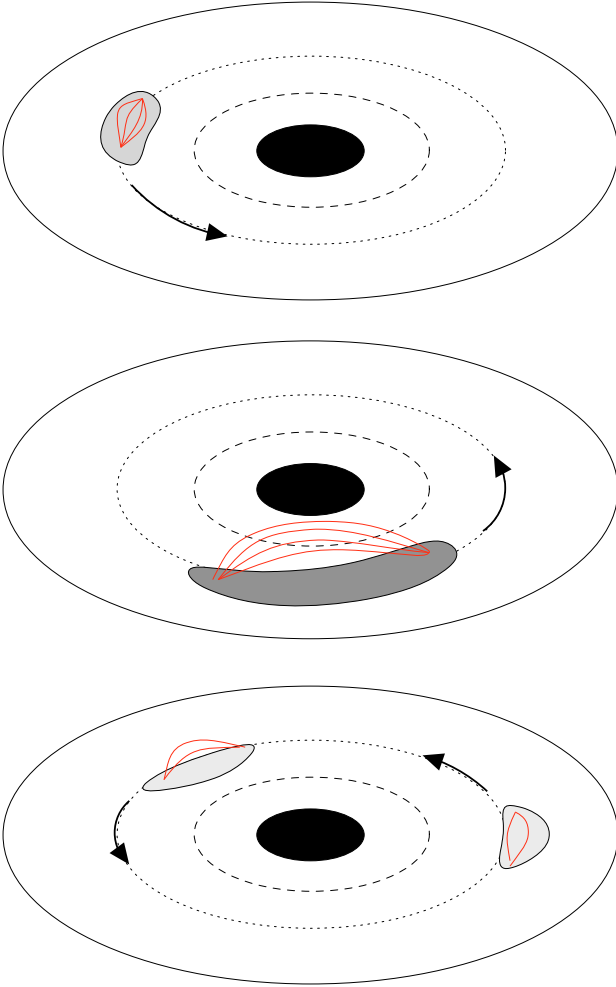
Fig. 10. Sketch of an expanding hot spot within an inclined temporary accretion disk of SgrA* based on Hawley & Balbus (1991; see also Balbus & Hawley 1998; and Balbus 2003). The black center indicates the event horizon of the massive black hole, the solid line the outer edge of the accretion disk (see e.g. Meyer et al. 2005). The long dashed line marks the inner last stable orbit. The dotted line represents a random reference orbit to show the effect of differential rotation of an extended emission region. The red solid line across the grey shaded extended spots depicts the magnetic field lines that through magneto-hydrodynamical instabilities provide a coupling between disk sections at different radii.
