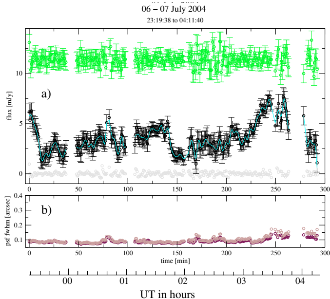
Fig. 2. Results of the re-reduction of the NIR 2.2 \mu\text{m} data from July 07, 2004. In panel a) the flux density scale is given in mJy. The top (green) data points represent the light curve of the nearby flux star S1 used for flux density calibration and the black data points with the blue interpolation line represent the SgrA* light curve. The time axis is given in minutes offset from the start time at 23:19:38 UT on 6 July 2004 and in UT hours at the bottom. In the bottom panel b) we show the FWHM of the PSF in the AO images that reflect the combination of AO correction and input seeing.
