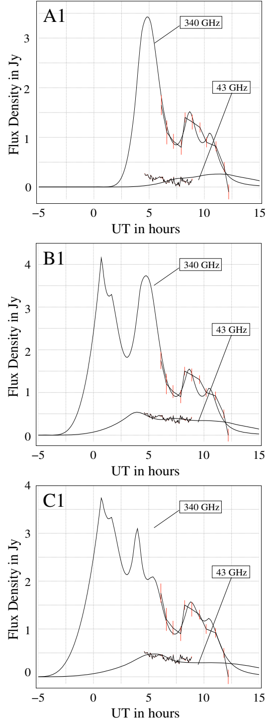
Fig. 7. The observed 43 GHz and 340 GHz light curves shown in comparison to model A1, B1, and C1. The data is shown with the offsets discussed in Sects. 2.3 and 2.4 removed.
