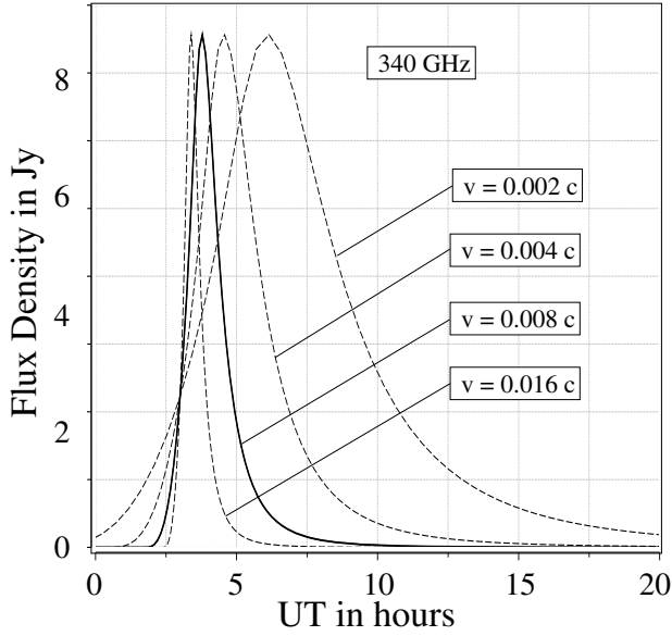
Fig. 4. A comparison of a 340 GHz light curve calculated with adiabatic expansion velocities that differ by factors of two.
