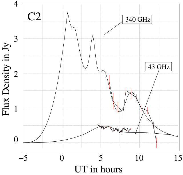
Fig. 8. The observed 43 GHz and 340 GHz light curves shown in comparison to model C2. The data is shown with the offsets discussed in Sects. 2.3 and 2.4 removed.
