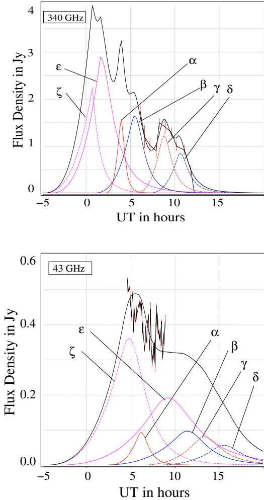
Fig. 6. Decomposition of the 340 GHz and 43 GHz light curve for model B1 (see Table 3) into the contributions of the different source components ( \alpha to \zeta ). The data are shown with the offsets discussed in Sects. 2.3 and 2.4 removed.
