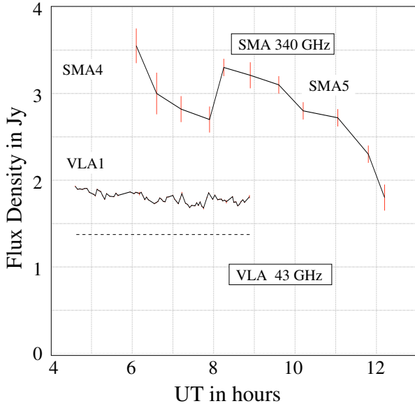
Fig. 3. The 340 GHz SMA and 43 GHz VLA total intensity light curves from July 07. The individual data points are connected by straight lines. The July 07 VLA data represent the excess flux density compared to the mean of the July 06 and 08 VLA data. The constant flux density of about 1.4 Jy that has to be added to this excess is indicated by a dashed line. For further details see text and Eckart et al. (2006a).
