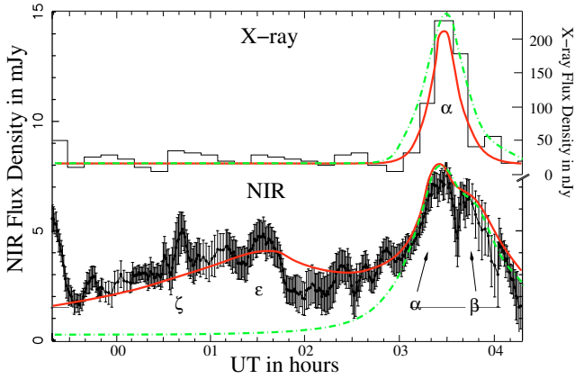
Fig. 9. A comparison between the X-ray and NIR 2.2 \mu\text{m} light curves shown in Fig. 1 and the modeling results for the A, B (both in green), and C (red) models. The contributions of individual model components as listed in Table 3 are labeled.
