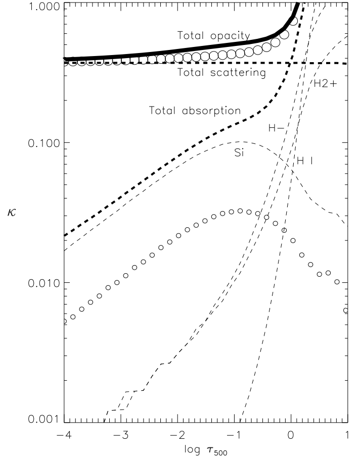
Fig. 5. Contributions to total continuous opacity around the 130 nm O I lines for a T_{\text{eff}} = 6500 , \log g = 4 , [\text{Fe}/\text{H}] = -3 model atmosphere. The absorption and the scattering part of total opacity are shown by the two thick dashed curves, as marked. For absorption, the importance of its main components (Si, \text{H}^- , \text{H}_2^+ and H I) is depicted. The total amount of continuous opacity is shown by the thick solid curve. For comparison, we also show (small circles) the reduced contribution of Si at [\text{Fe}/\text{H}] = -3.5 and consequent reduced total continuous opacity (large circles). The rest of the sources of opacity in the figure do not change significantly with this decrease in metallicity.
