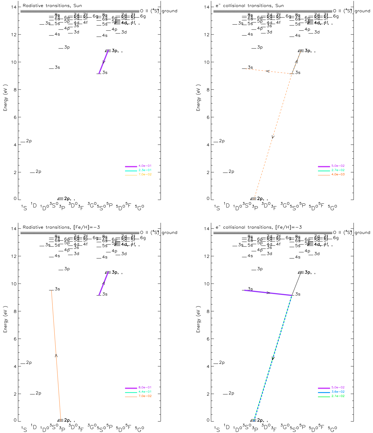
Fig. 4. Results from multi-MULTI runs for a solar model ( top panels ), and for a star with T_{\text{eff}} = 6500 K, \log g = 4.00 and [\text{Fe}/\text{H}] = -3 ( bottom panels ), when neglecting H collisions.
