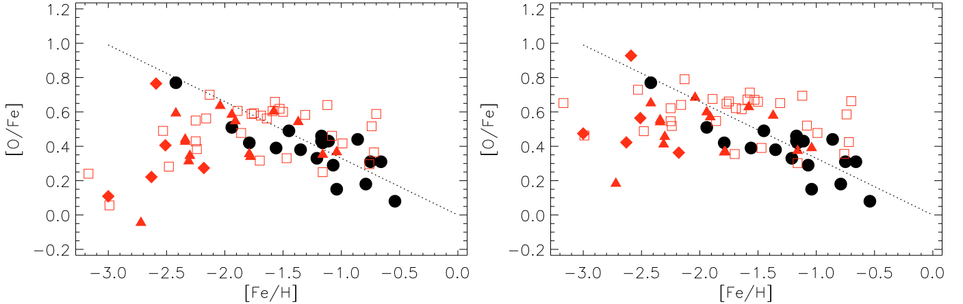
Fig. 10. Revised [O/Fe] versus [Fe/H] , from literature data. The different symbols are: filled circles, for [OI] -based, LTE-obeying values from Nissen et al. (2002); filled triangles, for the 1D estimates (from that same study, but non-LTE corrected according to our results) based on the O I 777 nm triplet; filled diamonds for OI-based values for the stars in Israelian et al. (2001) with fully determined stellar parameters and oxygen triplet abundances in their study, taking into account our non-LTE corrections on the oxygen triplet; and empty squares, for our non-LTE corrected estimates using the Meléndez et al. (2006) data set (after adjusting T_{\text{eff}} -scale, see Nissen et al. 2007). The non-LTE abundance corrections we applied were computed with a choice of S_H = 0 and S_H = 1 (left and right panel respectively) for hydrogen collisions. The dotted line indicates the mean trend suggested by Israelian et al. (2001), i.e. [O/Fe] = -0.33 [Fe/H] .
