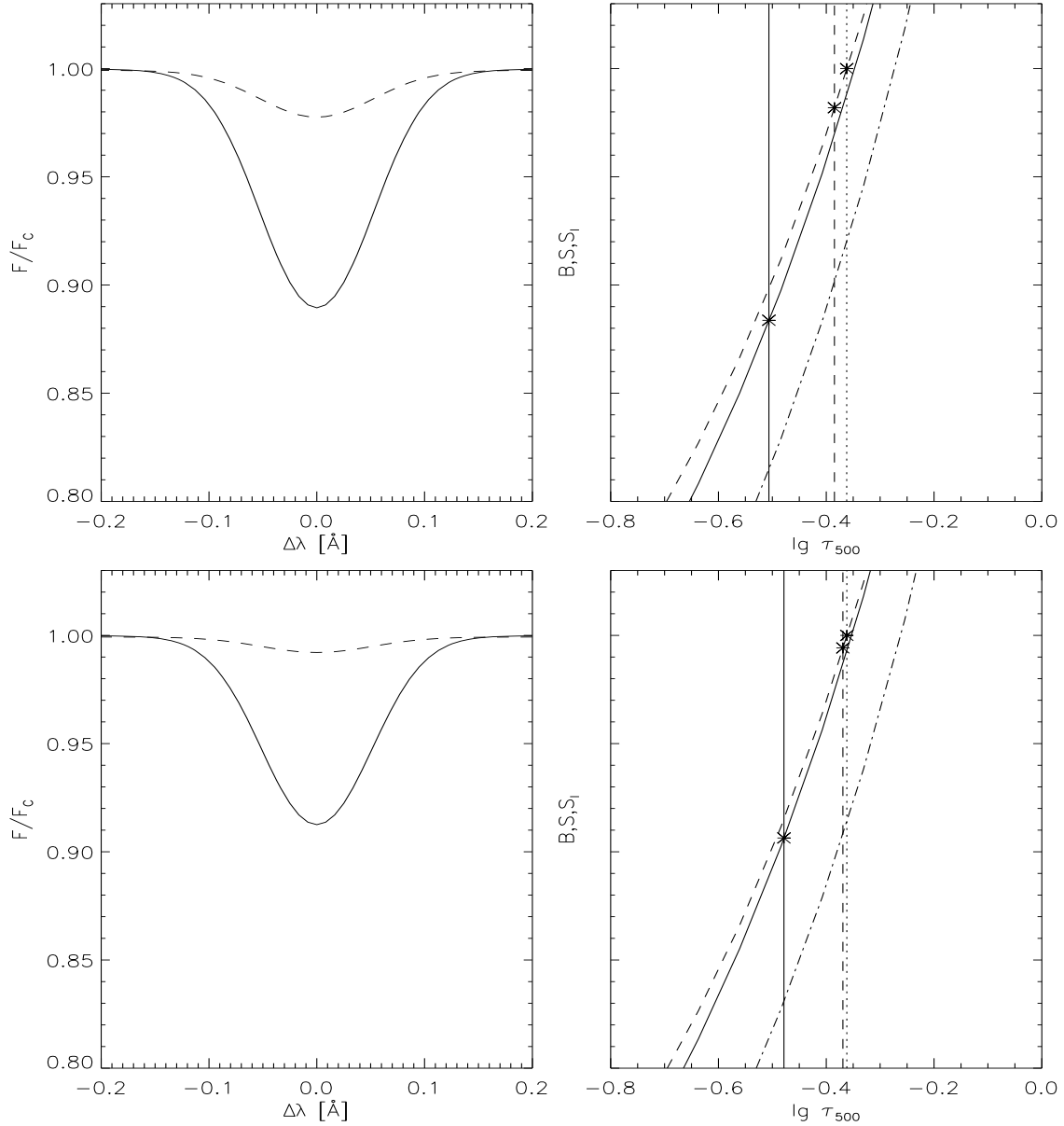
Fig. 3. The oxygen feature at 777.2 nm (the bluest and strongest of the O I triplet lines), for [\text{Fe}/\text{H}] = -3.00 (top panels) and -3.50 (bottom panels). The atmospheric models have T_{\text{eff}} = 6500 K, \log g = 4.00 [cgs] and solar-scaled, alpha-enhanced ( [\alpha/\text{Fe}] = +0.4 ) abundances. The case with no hydrogen collisions is shown here. Top left: the resulting LTE (dashed curve) and non-LTE (solid curve) flux profiles normalized to continuum flux, for the spectral feature considered. Top right: normalized values of B (dashed), S (solid) and S_1 (dash-dot). The vertical scale in the two cases is therefore the same. The left panel illustrates how at low metallicity the line becomes much stronger in non-LTE compared to LTE. In the right panel , the starred symbols show fluxes corresponding to the Eddington-Barbier formation height, the latter being indicated by vertical dotted, dashed and solid lines (respectively for continuum, LTE line center, and non-LTE line center). Note that the Eddington-Barbier value is \tau_{\nu}^{\text{cont}} = 2/3 exactly when the source function varies linearly with optical depth, while it is slightly smaller in this case. The right panel shows that at low metallicity the source function effect is small. Bottom: as above, but for [\text{Fe}/\text{H}] = -3.50 .
