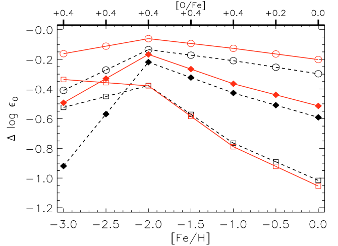
Fig. 7. Non-LTE abundance corrections versus metallicity, for the strongest O I IR 777 nm triplet line. The lines connect models with given T_{\text{eff}} and \log g but varying metallicity. Different symbols denote, respectively, results for models representative of a normal dwarf ( T_{\text{eff}} = 5780 K, \log g = 4.44 , indicated by open circles), a normal turn-off star ( T_{\text{eff}} = 6500 K, \log g = 4 , marked with filled diamonds) and a RR-Lyrae star ( T_{\text{eff}} = 6500 K, \log g = 2 , indicated by open squares). Dashed lines are for no H collisions, solid lines for a choice of S_{\text{H}} = 1 . Solar-scaled oxygen abundance with \alpha -enhancement below solar metallicity was adopted in the calculations, as indicated by the horizontal axis at the top of the figure.
