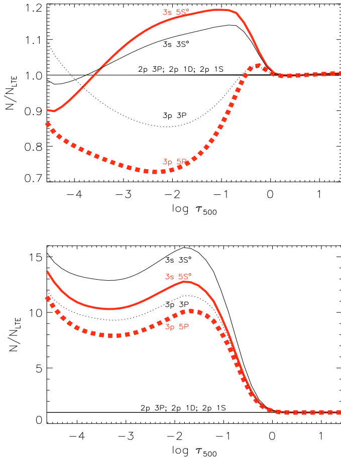
Fig. 2. Departure coefficients in the level population of the lowest energy levels (up to 3p\ ^3P ) in our oxygen model atom (for the case without H collisions) are shown respectively for the Sun ( upper panel ) and a metal-poor turn-off atmospheric model with [\text{Fe}/\text{H}] = -3 ( lower panel ). Note the very different scales for the y -axes in the two panels. The thicker lines indicate the departure coefficients for lower and upper levels (solid and dashed curve respectively) in the 777 nm triplet. Note that only one curve is plotted for the latter levels, because the small differences in the departure coefficients among those fine structure levels does not play an important role here.
