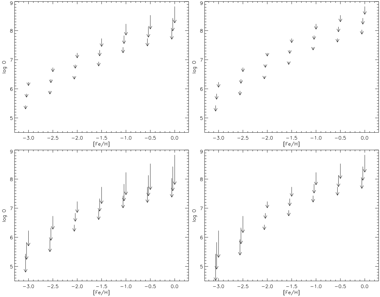
Fig. 8. Non-LTE abundance corrections versus metallicity, for the strongest O I IR 777 nm triplet line. Top: T_{\text{eff}} = 5500 K; \log g = 2 ( left panel ) and \log g = 4 ( right panel ) respectively. Bottom: same, but for T_{\text{eff}} = 6500 K. Results shown in all four panels are computed neglecting collisions with H atoms. The non-LTE corrections tend to become large at high temperature, both in dwarfs and giants. They are significant also in cooler solar-metallicity giants.
