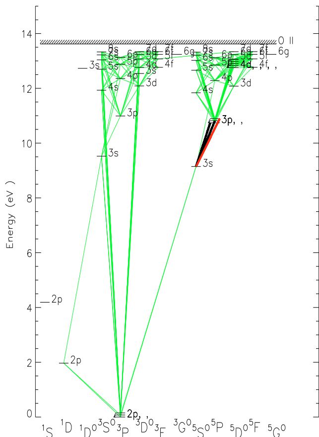
Fig. 1. Grotrian diagram of the atomic model we employed, showing the 53 energy levels of neutral oxygen and the single first ionization level. Lines connecting the various levels in the figure represent the 208 radiative bound-bound transitions included in the model. The 777 nm transitions are marked with thicker lines.
