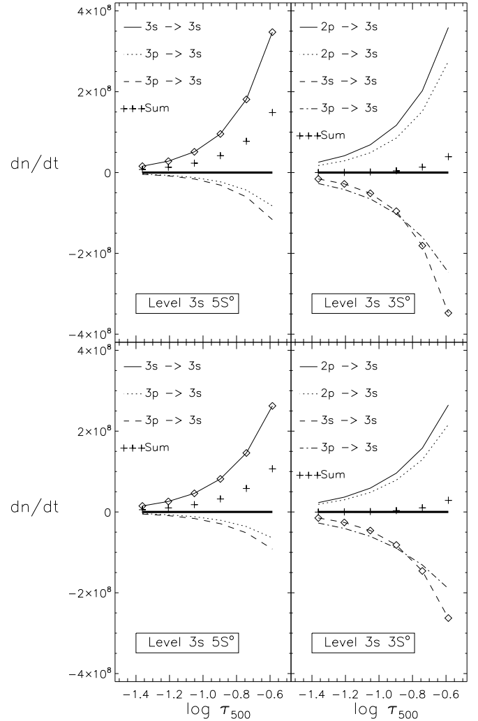
Fig. 6. Net rates contributing to the balance of levels 3s\ ^5\text{S}^{\circ} (left) and 3s\ ^3\text{S}^{\circ} (right). Lines with and without diamond symbols indicate the contribution to a given rate from collisions, and that from radiation, respectively. Only the rates with large influence on the level population are shown (their summed contribution is represented by crosses). The thick horizontal line at dn/dt = 0 marks the statistical equilibrium expectation that the total sum of all rates to and from a given level is equal to zero. The atmospheric model has T_{\text{eff}} = 6500 , \log g = 4 and \log \epsilon_0 = 6.5 . Plots are for [\text{Fe}/\text{H}] = -3 (upper panels) and -3.5 (lower panels) respectively.
