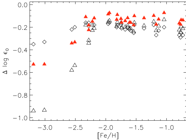
Fig. 9. Non-LTE abundance corrections versus metallicity, for the O I IR 777 nm triplet. Open diamonds indicate the results of Meléndez et al. (2006), while the other symbols mark our corrections for S_H = 0 and S_H = 1 (open and filled triangles respectively).
