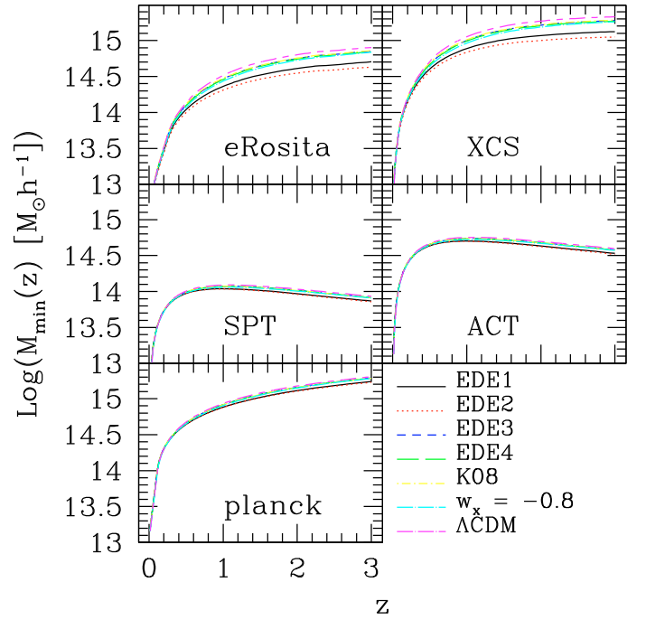
Fig. 2. The minimum mass for clusters included in the catalogs constructed with the five different surveys investigated in this work, as labelled in the plot. Results for the seven different dark-energy models described in the text are shown, using the same color and line types as in Fig. 1.
