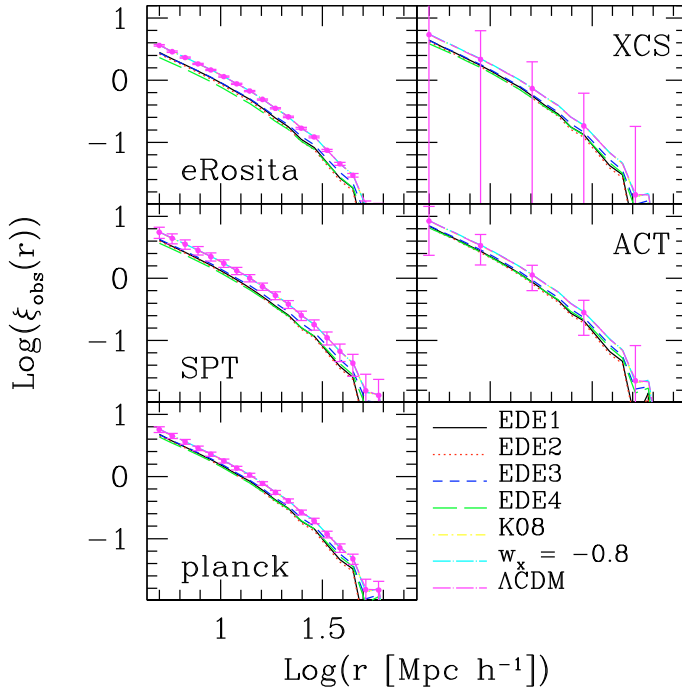
Fig. 5. Predicted correlation function for the five cluster catalogs used in this work. Different colors and linestyles refer to different cosmological models, as labelled in the plot. Errorbars are computed with the bootstrap method, and refer only to the \Lambda\text{CDM} model for clarity.
