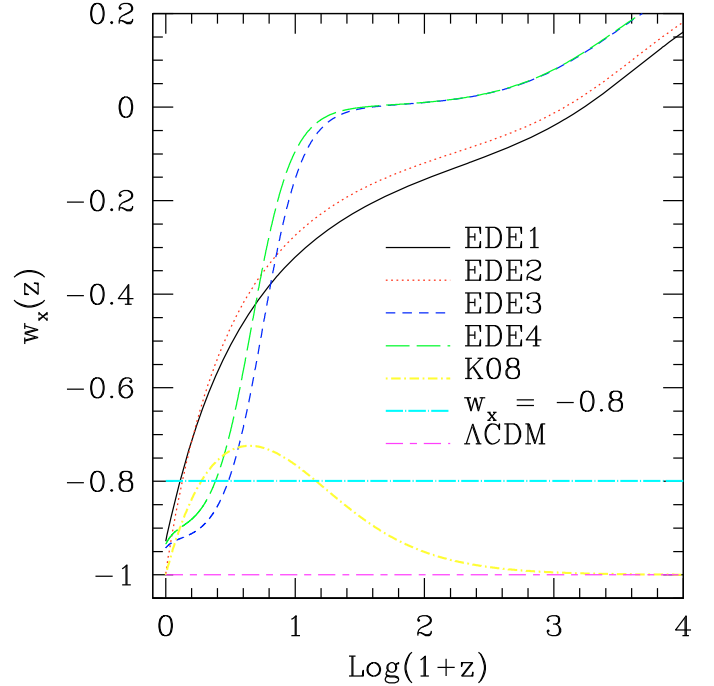
Fig. 1. The redshift evolution of the dark energy equation of state parameter w_x for the seven dark energy models adopted in this work, as labelled in the plot.
