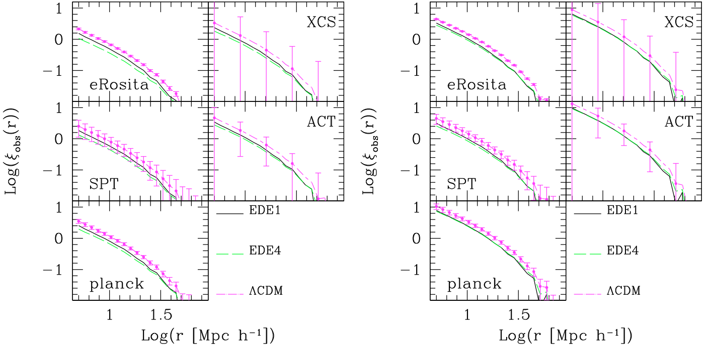
Fig. 7. Same as Fig. 5 but with cluster catalogs restricted to z \leq 0.1 (left panel) and z > 0.1 (right panel). For the SPT catalog, the right panel actually shows the restriction to 0.1 < z \leq 0.3 . Only three cosmological models are shown here for simplicity.
