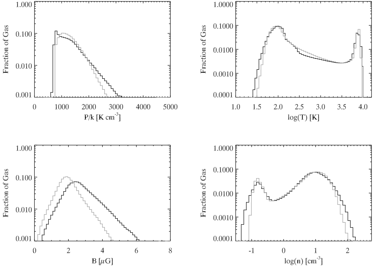
Fig. 3. Comparison of pressure, temperature, magnetic field and density PDFs, averaged over the final two orbits of the simulation. The dark line is for ZEUS, and the light line for NIRVANA. Generally the agreement is quite good, but there are some differences worth noting. For ZEUS the distributions of pressure, temperature, and density all extend to both higher and lower values as compared to NIRVANA. We also note the slightly larger fraction of unstable gas in the temperature PDF. Finally, the peak of the magnetic field PDF of ZEUS is shifted to slightly higher values, and extends much farther towards higher values of B .
