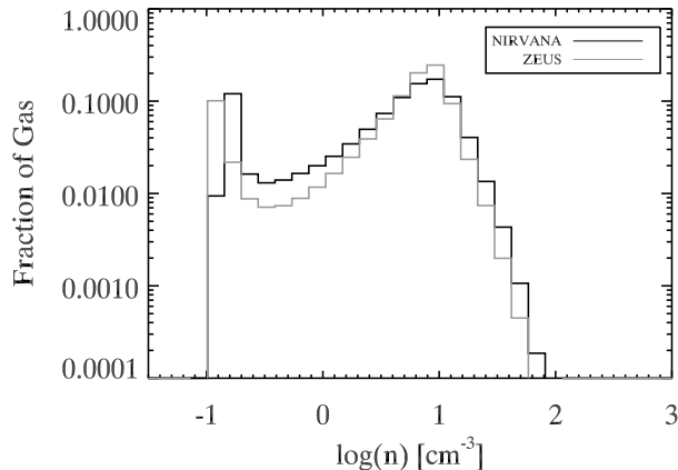
Fig. 6. Mass-weighted density PDFs for NIRVANA and ZEUS averaged over the second half of the simulation for the forced TI simulation.
