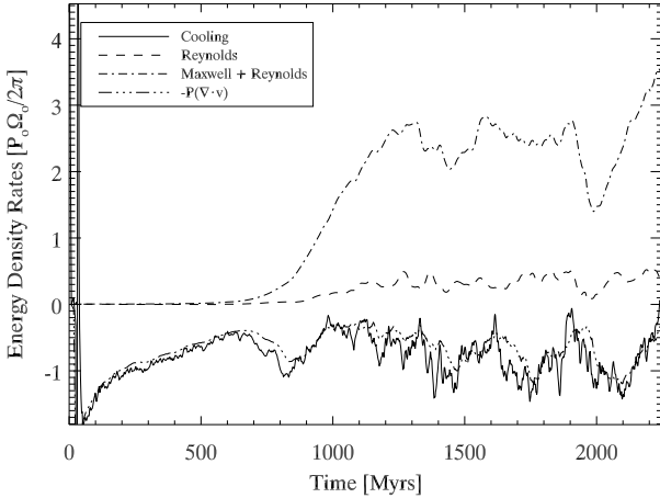
Fig. 2. We plot the same quantities as shown in Fig. 1, but for the non-conservative NIRVANA run. In this case the net heating/cooling term has the opposite sign as was found for the conservative NIRVANA run, and is now well correlated with the -P(\nabla \cdot v) term.
