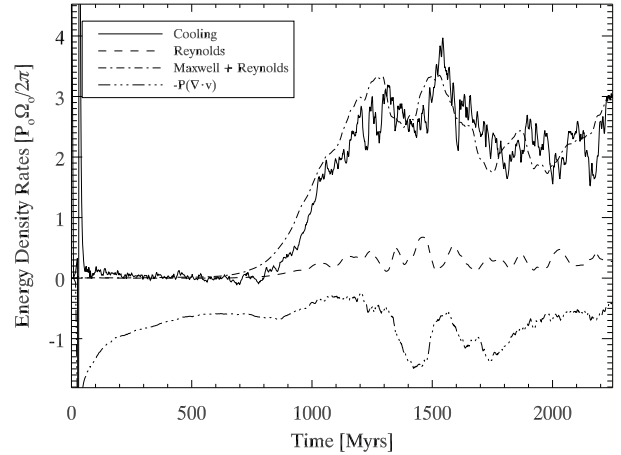
Fig. 1. We plot, for the conservative NIRVANA run, the net energy gain/loss rate from the net heating/cooling function, the volume-averaged energy density input rates for the Reynolds stress, and the sum of the Maxwell and Reynolds stresses, as well as the -P(\nabla \cdot v) term. A positive value of the cooling term implies net cooling is occurring in the simulation.
