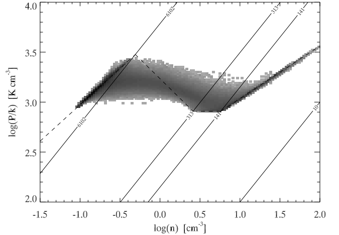
Fig. 5. Same as plotted in Fig. 4, but for the conservative NIRVANA run. Compared to ZEUS, gas in the warm stable phase does not extend to as high temperatures, and gas in the cold phase does not extend to as cool temperatures. The unstable region, however, is significantly broadened, most notably between 141 K and 313 K to higher pressure and higher density.
