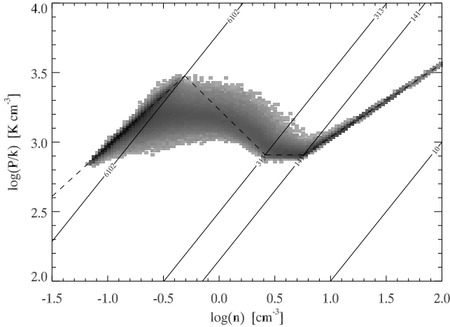
Fig. 4. Phase-space diagram of pressure and density for ZEUS, where intensity indicates the relative fraction of gas at a particular density and pressure. The dashed line represents thermal equilibrium, when heating and cooling rates are equal. The solid diagonal lines are contours of constant temperature, and are labeled individually. These temperatures correspond to those that define the transitions for the piece-wise continuous cooling function. The majority of the gas exists in thermal equilibrium in the warm and cold phases.
