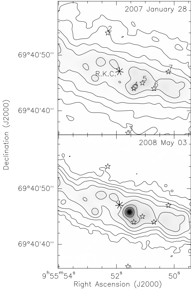
Fig. 2. Contours and grey scale represent 22.2 GHz images of the central region of M 82 taken on 2007 January 28 ( top ) and 2008 May 03 ( bottom ). The new bright source is very conspicuous in the latter image. Contour values are -4, 4, 8, 16, 32, 64, 128, 256, and 512 times 0.2 \text{ mJy beam}^{-1} , roughly the (comparable) rms noise level in both images. The star symbols mark the positions of the X-ray sources discussed by Matsumoto et al. (2001) and in the top panel bear these authors' nomenclature. The asterisk gives the position of the radio kinematic center (R.K.C.) of M 82 as determined by Weliachew et al. (1984) . Both images were restored with a circular beam of 1.5 \text{ arcsec} . Since the observation on 2007 January 28 was made in C configuration, there was much more data from short baselines, which results in better sensitivity to extended emission.
