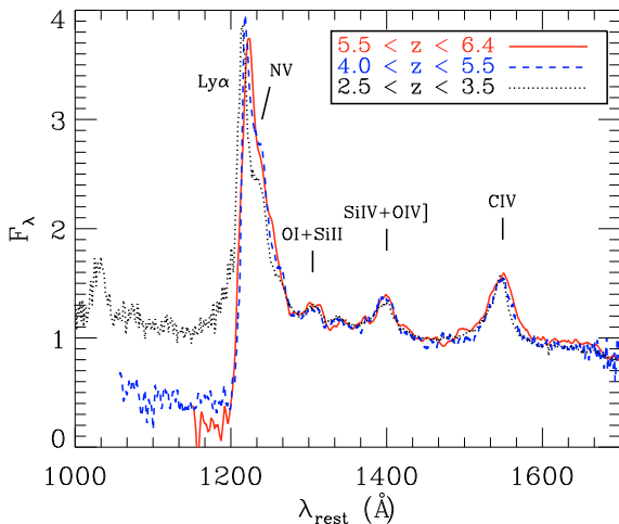
Fig. 2. Stacked spectra of quasars in different redshift bins (all normalized to \lambda = 1450 \text{ \AA} ). The red solid line and the blue dashed line are the stacked spectra from our sample in the redshift intervals 5.5 < z < 6.4 and 4.0 < z < 5.5 , respectively. The black dotted line is the SDSS quasars stacked spectrum in the redshift interval 2.5 < z < 3.5 .
