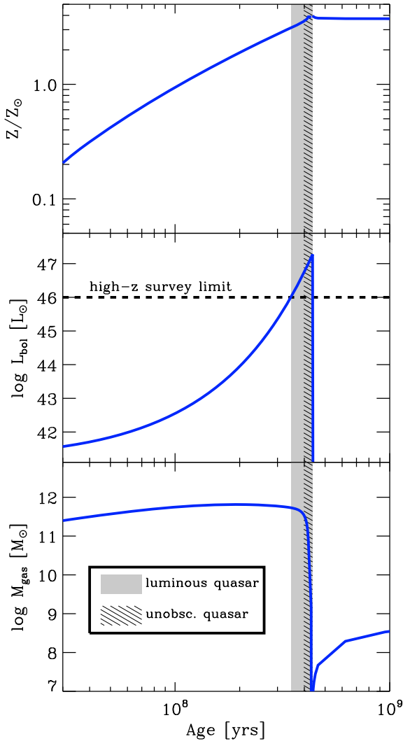
Fig. 3. Evolution of the gas metallicity ( top ), bolometric quasar luminosity ( middle ) and total gas mass ( bottom ) in the model by Granato et al. (2004). The horizontal dashed line shows the approximate minimum bolometric luminosity detectable at high- z in the SDSS quasar survey. The shaded area shows the epoch when a high- z quasar is luminous enough to be detected in the SDSS survey (if unobscured). The hatched area is the epoch when the quasar has ejected more than half of the gas mass, and it is likely unobscured and therefore detectable in optical surveys. By the time the quasar has reached the luminous, “unobscured” epoch the gas is already highly enriched.
