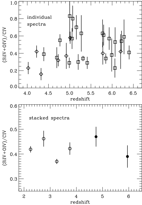
Fig. 1. (Upper) (SiIV+OIV)/CIV flux ratio as a function of redshift for quasars observed in this work. Squares indicate non-BAL quasars, while diamonds indicate BAL quasars. (Lower) (SiIV+OIV)/CIV ratio inferred from quasar stacked spectra, both for the high-redshift quasars presented here (filled symbols) and for the lower redshift quasars studied in Nagao et al. (2006a) (empty symbols).
