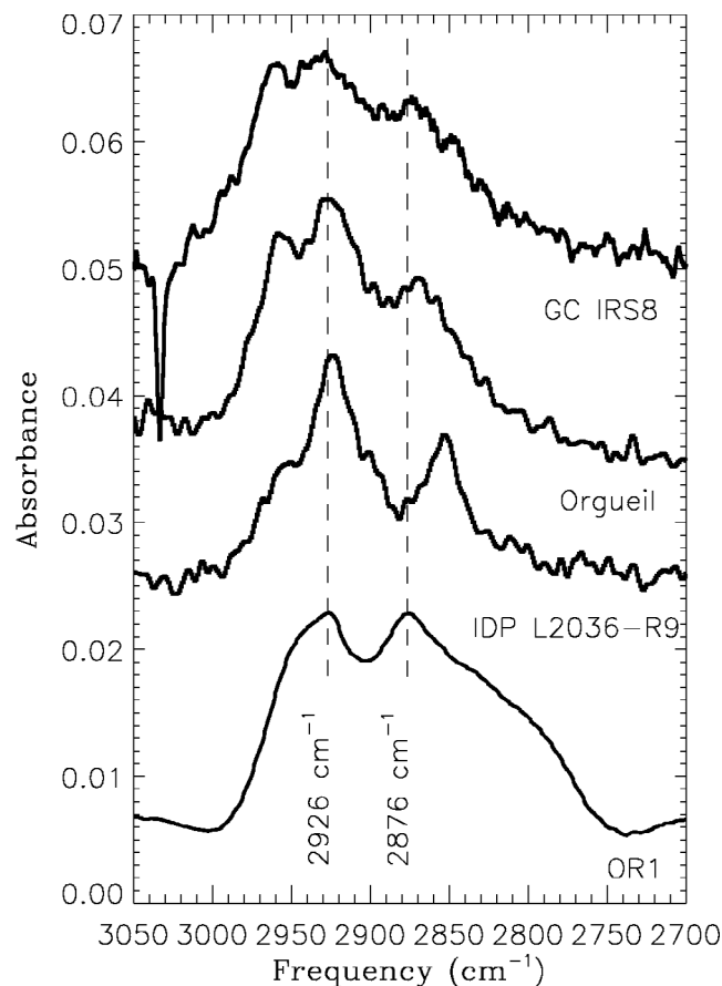
Fig. 6. Comparison of the infrared 3.4 \mu\text{m} features corresponding to an organic refractory residue (OR1, see Sect. 3.1), an IDP named L2036-R9, the Orgueil residue obtained from hydrolysis, and the Galactic Center source GC IRS8.
