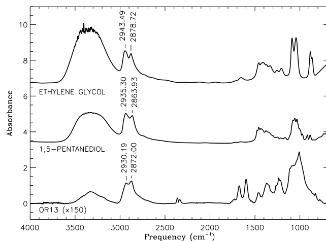
Fig. 3. Comparison between OR13 spectrum (bottom trace) and two alcohols, 1,5-pentanediol (middle trace) and ethylene glycol (top trace). The spectra were obtained at room temperature.
