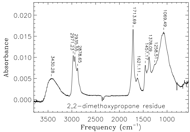
Fig. 5. Top: spectrum corresponding to deposition of 2,2-dimethoxypropane ice. Bottom: spectrum of residue made by simultaneous deposition and UV-irradiation of 2,2-dimethoxypropane, followed by warm-up to room temperature. The band between 2400–2300 \text{cm}^{-1} is \text{CO}_2 gas absorbing along the beam of the infrared spectrometer.
