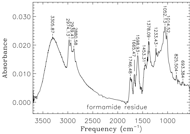
Fig. 4. Top: spectrum corresponding to deposition of formamide ice. Bottom: spectrum of residue made by simultaneous deposition and UV-irradiation of formamide, followed by warm-up to room temperature.
