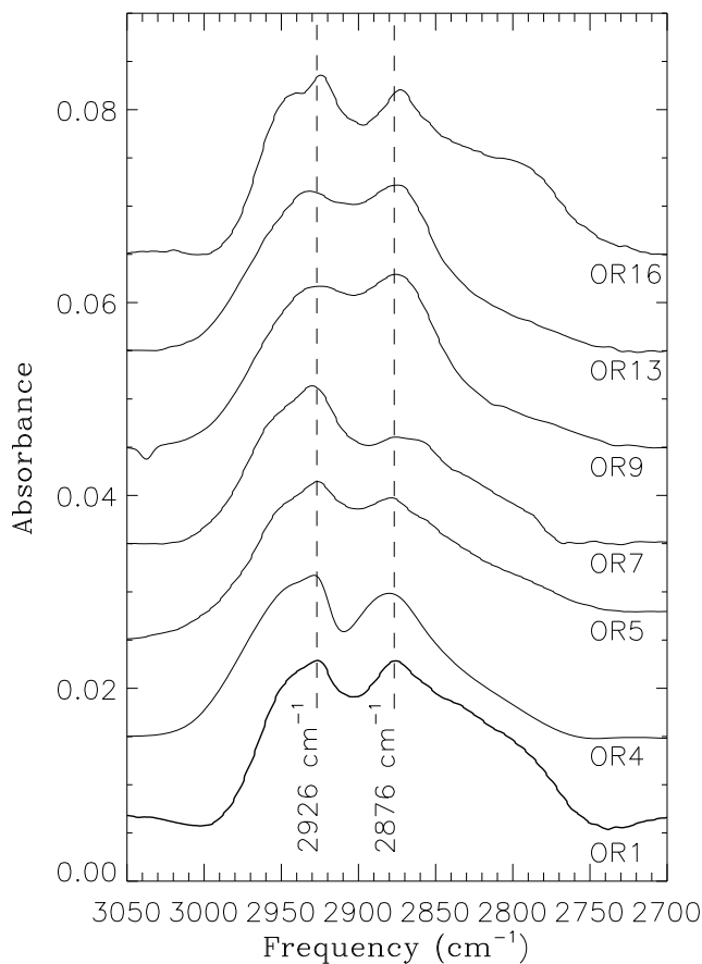
Fig. 1. Organic refractory residue spectra from photoprocessing of different ice mixtures. See Table 1 for experimental parameters of the samples.
