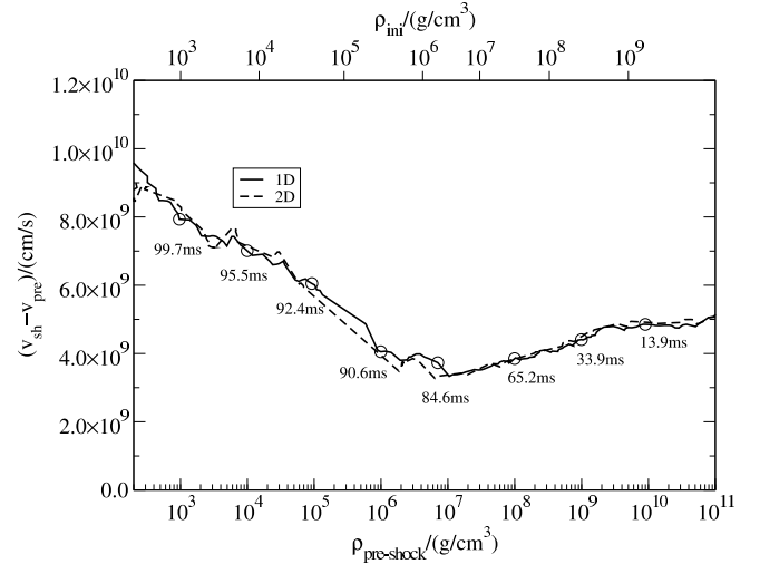
Fig. 9. Velocity of the shock, v_{\text{sh}} , relative to the preshock gas, whose velocity is v_{\text{pre}} , versus preshock density as obtained from the 1D (solid line) and 2D (dashed line) simulations. Post-bounce times of the 1D run are indicated by the labeled open circles (as in Figs. 6 and 8). For orientation, the scale on the upper horizontal axis approximately gives the initial densities of the progenitor model. These are smaller than the values on the lower horizontal axis for layers which have started to collapse before they are reached by the outgoing shock.
