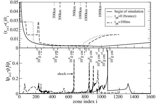
Fig. 2. Radial resolution of the 1D simulation at the beginning of the simulation, at core bounce, and 100 ms after core bounce. The upper panel shows the relative radius variation, |\Delta r|/r , the lower panel the relative density difference, \Delta\rho/\rho , between neighboring zones as a function of the radial zone index. Note that the radial grid is comoving with the fluid during collapse and is kept fix (i.e., Eulerian) after bounce, but then is still refined by adding more zones between bounce and 100 ms later (for reasons of better visibility only two times are given in the lower plot). In the panels the positions of selected radii and densities are marked by vertical bars in the same line styles as the curves. One can see that the radial spacing is better than 0.3% and the density change less than 10% in the region of the steep density gradient between about 10^0 \text{ g cm}^{-3} and 10^7 \text{ g cm}^{-3} .
