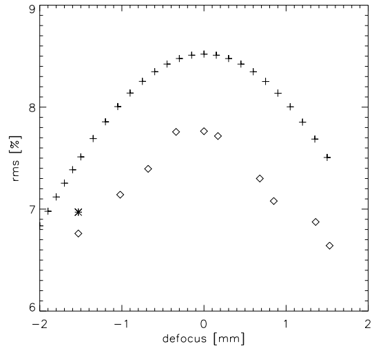
Fig. 3. Intensity contrast as a function of telescope defocus. Shown are results for a SP data set used taken on Jan. 16, 2007, 10:54:14–11:06:52 UT (diamonds) and the contrast values for the degraded simulation image (crosses). The value for the large map used to compare with the simulation is indicated by the asterisk, assuming that the location of the optimal focus was the same as for the other dataset. This also gives an indication of the observational uncertainty.
