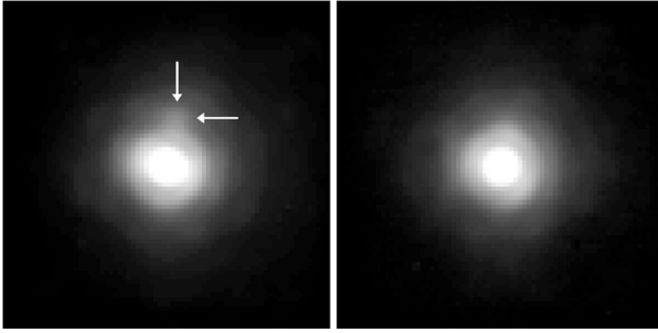
Fig. 1. NACO images of Achernar A and B ( left ) and \delta Phe ( right ) in the 2.17 \mu\text{m} filter obtained on 22 December 2007. The arrows indicate the position of Achernar B. The field of view is 1'' , and the grey scale is normalized for both images to the central part of the PSF.
