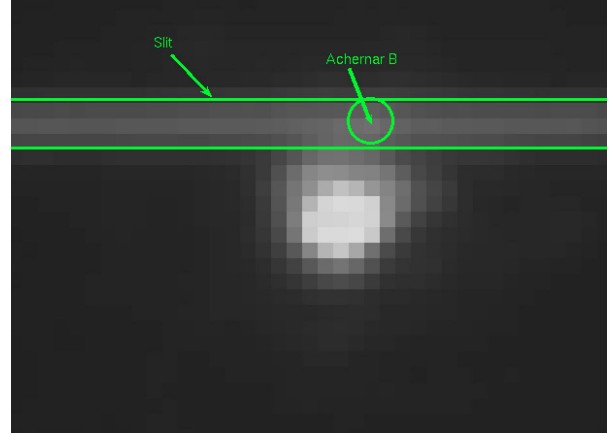
Fig. 4. Position of the NACO slit relative to Achernar A and B.
