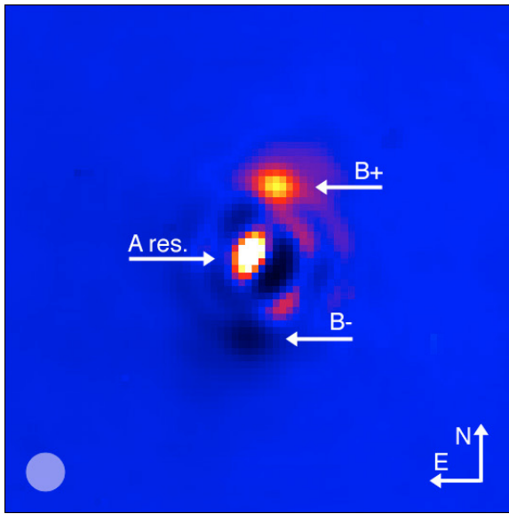
Fig. 2. Result of the subtraction of a 180^\circ rotated version of the image of the Achernar system presented in Fig. 1 ( left ) from itself. The “B+” and “B-” arrows point at the positions of the positive and negative images of Achernar B, and the “A res.” arrow indicates the A subtraction residuals. The aperture used for photometry is shown in the lower left corner, and the field of view is 1'' on each side.
