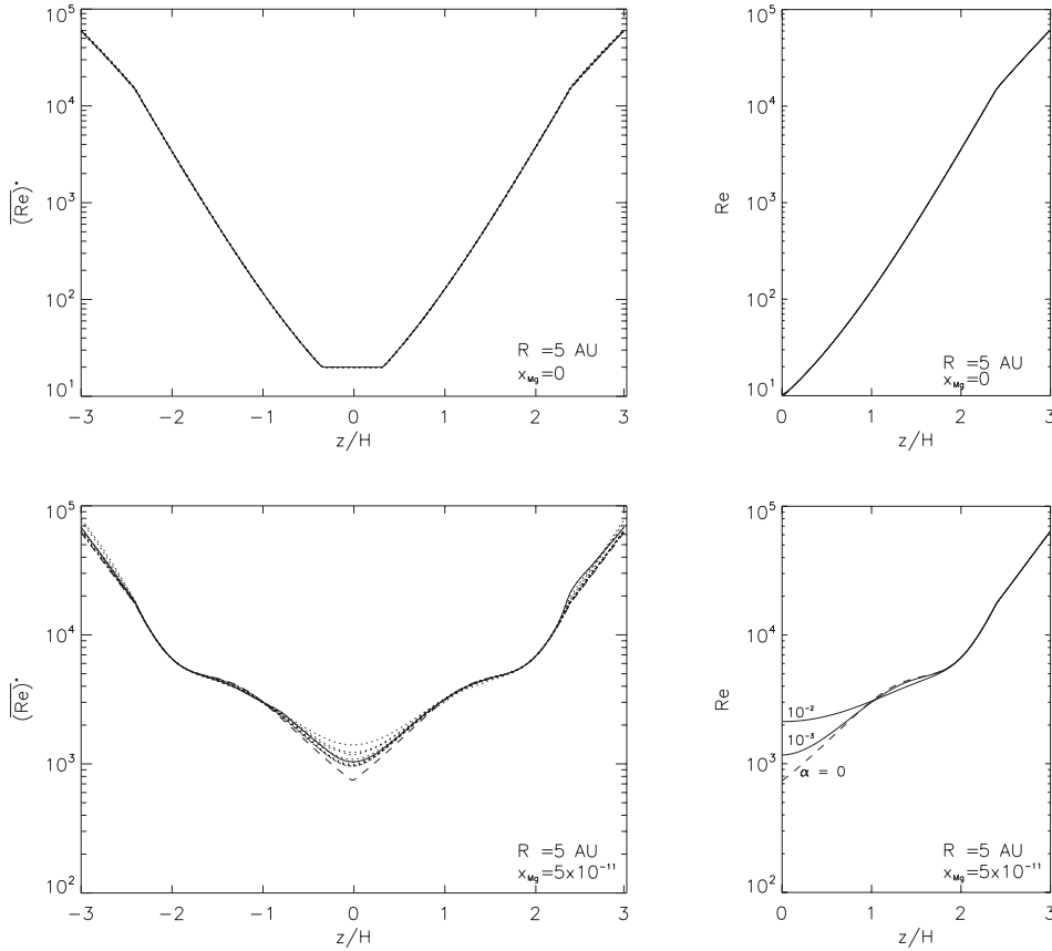
Fig. 8. model12: Comparison between vertical profiles of the magnetic Reynolds number obtained for R = 5 AU and x_{\text{Mg}} = 0 and x_{\text{Mg}} = 5 \times 10^{-11} , respectively. Left panels show shearing box simulation results, and right panels reaction-diffusion model results. In the left panels , the time averaged vertical profiles of the magnetic Reynolds number \overline{Re^*} are shown by taking the time average over 10 orbit intervals, starting from t = 0 (dashed line) towards [90, 100] (solid line). The other profiles (dotted lines) refer to the intervals t = [0, 10] , [10, 20] , \dots [80, 90] orbits. The resistivity profiles of the magnetic Reynolds number Re_m shown in the right panels refer to the equilibrium profiles obtained with the reaction-diffusion model assuming different values of \alpha_m . In particular for x_{\text{Mg}} = 0 , the value of the magnetic Reynolds number is not affected by the actual value of \alpha_m , leading to identical profiles for \alpha_m = 0 , \alpha_m = 10^{-3} , and \alpha_m = 10^{-2} . Note that both shearing box simulations and the reaction-diffusion models are initiated with the steady state profile obtained for \alpha_m = 0 .
