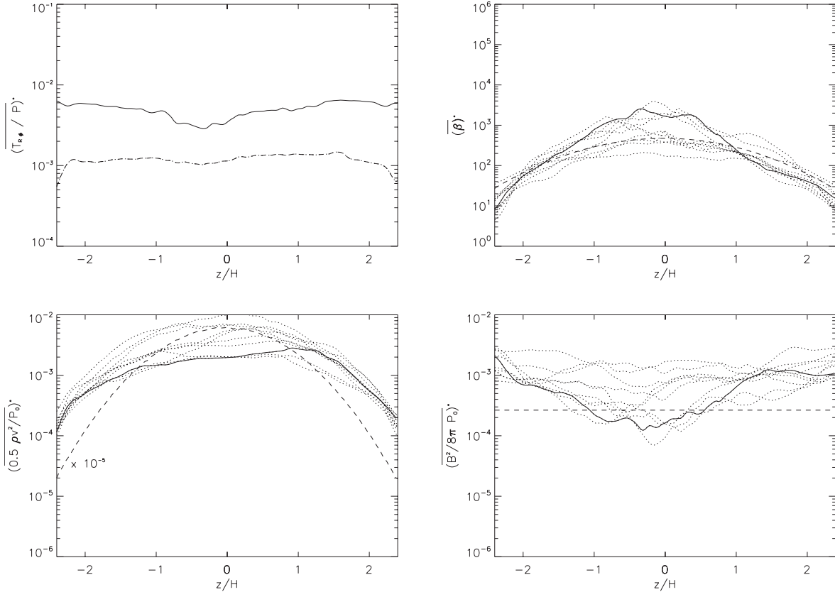
Fig. 5. model13: Time averaged vertical profiles of the horizontally averaged value of normalised Maxwell and Reynolds stresses T_{R\theta}/P_0 , the plasma parameter \beta , the kinetic energy 0.5\rho v^2/P_0 , and the magnetic energy B^2/(8\pi P_0) . As in the previous figures, the shearing box model is calculated for R = 10 AU and x_{\text{Mg}} = 5 \times 10^{-11} . \alpha_{\text{Max}} (solid line) and \alpha_{\text{Rey}} (dashed-dotted line) refer to a time average taken over [0, 100] orbits. For all the other quantities, the time average is taken over 10 orbit intervals, starting from t = 0 (dashed line) towards [90, 100] (solid line). The dotted lines refer to time averages taken over the intervals t = [0, 10] , [10, 20] , \dots , [80, 90] orbits.
