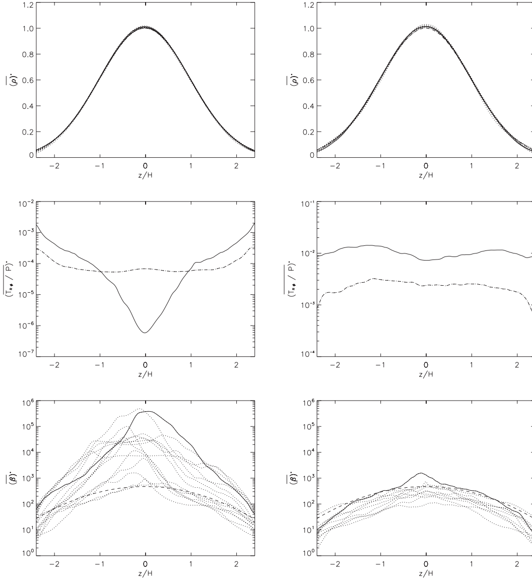
Fig. 3. model11/model12: Time averaged vertical profiles of the horizontally averaged density, normalised Maxwell and Reynolds stresses T_{R\phi}/P_0 , and plasma parameter \beta . The profiles on the left refer to the results obtained with the model assuming a fixed resistivity (model11). Results obtained with model12 are shown in the right panels. Both shearing box models are calculated for R = 10 AU and x_{\text{Mg}} = 5 \times 10^{-11} . \alpha_{\text{Max}} (solid line) and \alpha_{\text{Rey}} (dashed-dotted line) refer to a time average taken over [100, 200] orbits (for model11) and [0, 100] orbits for model12. For all the other quantities, the time averages are taken over 10 orbit intervals, starting from t = 0 (dashed line). For model11 the solid line denotes averages taken between t = [140, 150] orbits, and for model12 the solid lines represented averages taken between t = [90, 100] orbits. The dotted lines refer to time averages taken over t = [0, 10], [10, 20], \dots, [80, 90] for model12, \dots, [130, 140] for model11.
