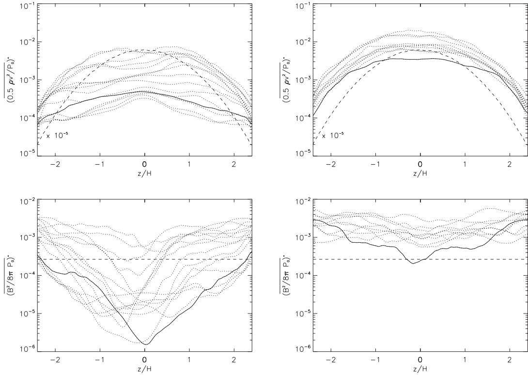
Fig. 4. model11/model12: Time averaged vertical profiles of the horizontally averaged kinetic energy, 0.5\rho v^2/P_0 , and the magnetic energy B^2/(8\pi P_0) . The profiles on the left panel show results obtained assuming a fixed resistivity profile (model11), while the results obtained with model12 are shown in the right panels . Both shearing box models are calculated for R = 10 AU and x_{\text{Mg}} = 5 \times 10^{-11} . The time average is taken over 10 orbit intervals, starting from t = 0 (dashed line) toward the interval t = [90, 100] (solid line, model12) and t = [140, 150] (solid line, model11), respectively. The dotted lines refer to time averages taken over t = [0, 10], [10, 20], \dots, [80, 90], [130, 140] orbits.
