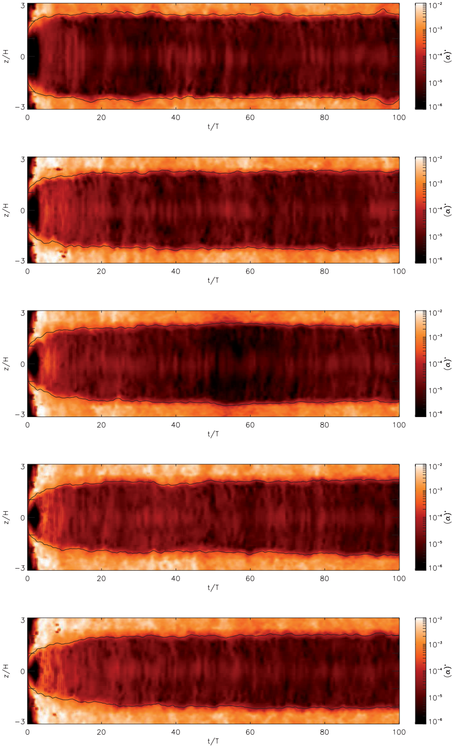
Fig. 6. model12: Space-time plots of the horizontally averaged value of \alpha calculated at different radial positions R and a metal elemental abundance of x_{\text{Mg}} = 0 . The cylindrical radius R varies from 1 AU ( top panel ) to 10 AU ( bottom panel ) passing through R = 3, 5, and 7 AU. The solid line drawn at the boundary between the live and dead zones indicates the position where the horizontally averaged Lundquist number Lu = 1 .
