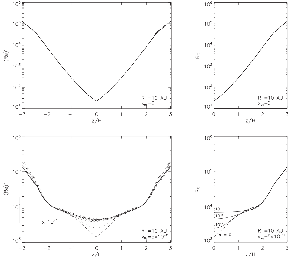
Fig. 10. mode12: Comparison between vertical profiles of the magnetic Reynolds number obtained for R = 10 AU and x_{\text{Mg}} = 0 and x_{\text{Mg}} = 5 \times 10^{-11} , respectively. Left panels show shearing box simulation results, and right panels reaction-diffusion model results. In the left panels , the time averaged vertical profiles of the magnetic Reynolds number \overline{Re} are shown by taking the time average over 10 orbit intervals, starting from t = 0 (dashed line) towards [90, 100] (solid line). The other profiles (dotted lines) refer to the intervals t = [0, 10], [10, 20], \dots [80, 90] orbits. The resistivity profiles of the magnetic Reynolds number Re_m shown in the right panels refer to the equilibrium profiles obtained with the reaction-diffusion model assuming different values of \alpha_m . In particular for x_{\text{Mg}} = 0 , the value of the magnetic Reynolds number is not affected by the actual value of \alpha_m , leading to identical profiles for \alpha_m = 0, \alpha_m = 10^{-3} , and \alpha_m = 10^{-2} . Note that both shearing box simulations and the reaction-diffusion models are initiated with the steady state profile obtained for \alpha_m = 0 .
