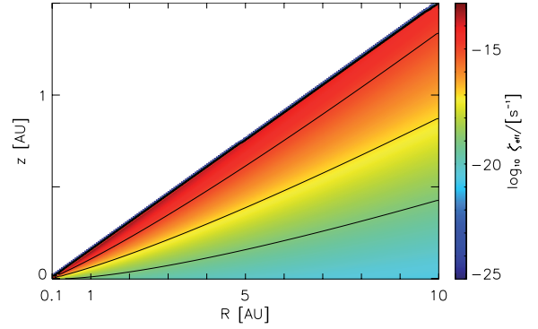
Fig. 1. The effective X-ray ionisation rate \zeta_{\text{eff}} per hydrogen nucleus. The contour lines refer to values of \zeta_{\text{eff}} : 10^{-15} , 10^{-17} , and 10^{-19} \text{s}^{-1} .
