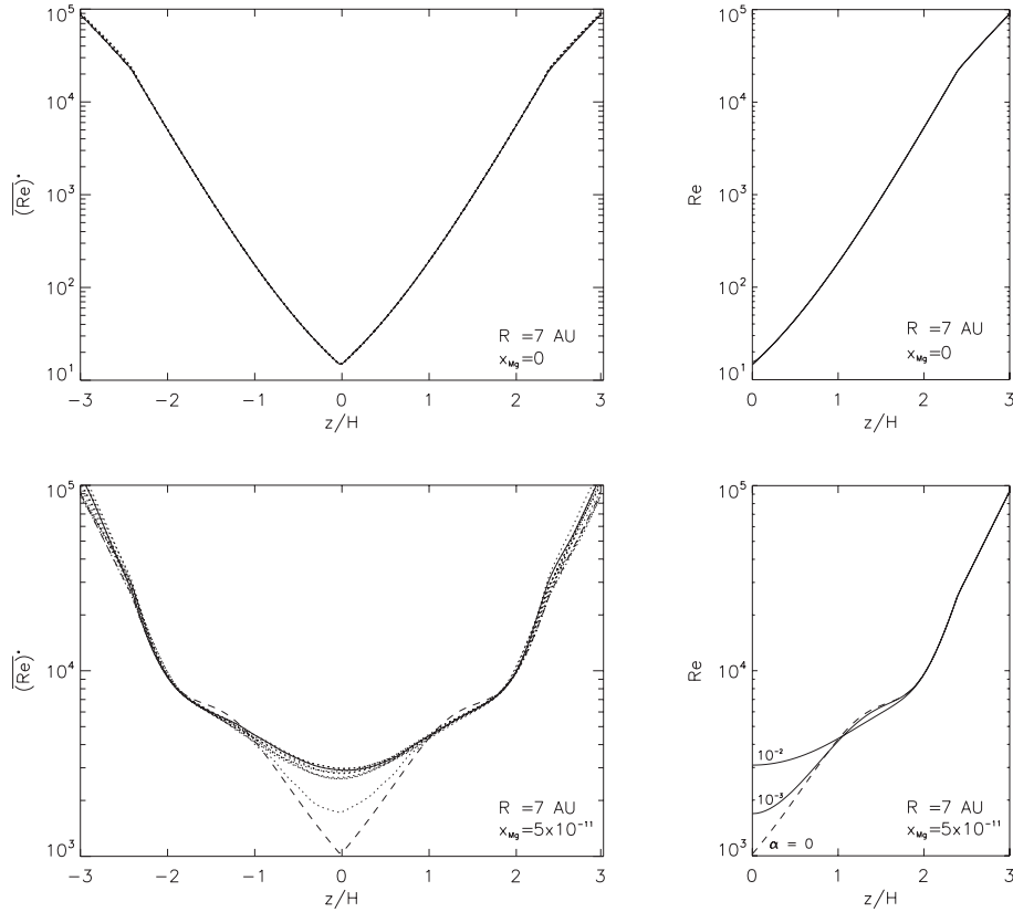
Fig. 9. model2: Comparison between vertical profiles of the magnetic Reynolds number obtained for R = 7 AU and x_{\text{Mg}} = 0 and x_{\text{Mg}} = 5 \times 10^{-11} , respectively. Left panels show shearing box simulation results, and right panels reaction-diffusion model results. In the left panels , the time averaged vertical profiles of the magnetic Reynolds number \overline{Re^*} are shown by taking the time average over 10 orbit intervals, starting from t = 0 (dashed line) towards [90, 100] (solid line). The other profiles (dotted lines) refer to the intervals t = [0, 10] , [10, 20] , \dots , [80, 90] orbits. The resistivity profiles of the magnetic Reynolds number Re_m shown in the right panels refer to the equilibrium profiles obtained with the reaction-diffusion model assuming different values of \alpha_m . In particular for x_{\text{Mg}} = 0 , the value of the magnetic Reynolds number is not affected by the actual value of \alpha_m , leading to identical profiles for \alpha_m = 0 , \alpha_m = 10^{-3} , and \alpha_m = 10^{-2} . Note that both shearing box simulations and the reaction-diffusion models are initiated with the steady state profile obtained for \alpha_m = 0 .
