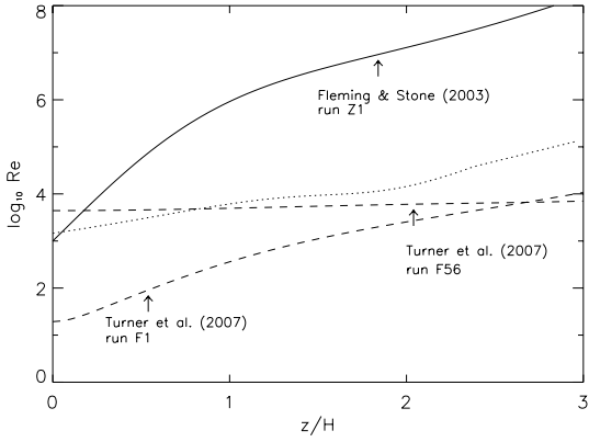
Fig. 2. Vertical profiles of the magnetic Reynolds numbers Re_m . The profile drawn with the solid line refers to the profile used by Fleming & Stone (2003) in their model with a small dead zone. The two dashed lines correspond to profiles used by Turner et al. (2007) in their models F1 and F56. The profile drawn with the dotted line refers to our mode11, calculated at R = 10 AU and a metal abundance of x_{\text{Mg}} = 5 \times 10^{-11} . Details are discussed in the text.
