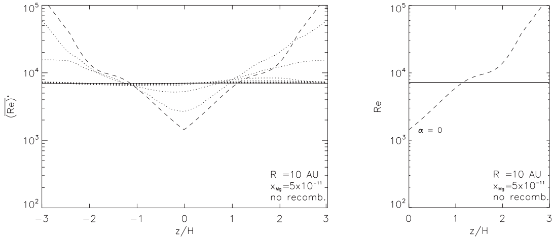
Fig. 11. mode13: Comparison between vertical profiles of the magnetic Reynolds number obtained for R = 10 AU and x_{\text{M}} = 5 \times 10^{-11} obtained by the shearing box simulation ( left panel ) and the reaction-diffusion model ( right panel ). The results refer to the simulation where recombination and ionisation are switched off (mode13). In the left panel , the time averaged vertical profiles of the magnetic Reynolds number \overline{Re}_m^* are shown by taking time averages over 10 orbit intervals, starting from t = 0 (dashed line) towards [90, 100] (solid line). The other profiles (dotted lines) refer to t = [0, 10], [10, 20], \dots [80, 90] . The resistivity profiles of the magnetic Reynolds number Re_m shown in the right panel refer to the equilibrium profiles obtained with the reaction-diffusion model assuming different values of \alpha_m . In fact, the equilibrium profile obtained for mode13 is not affected by the actual value of \alpha_m > 0 . Note that both shearing box simulation and the reaction-diffusion model are initiated with the equilibrium profile obtained for \alpha_m = 0 .
