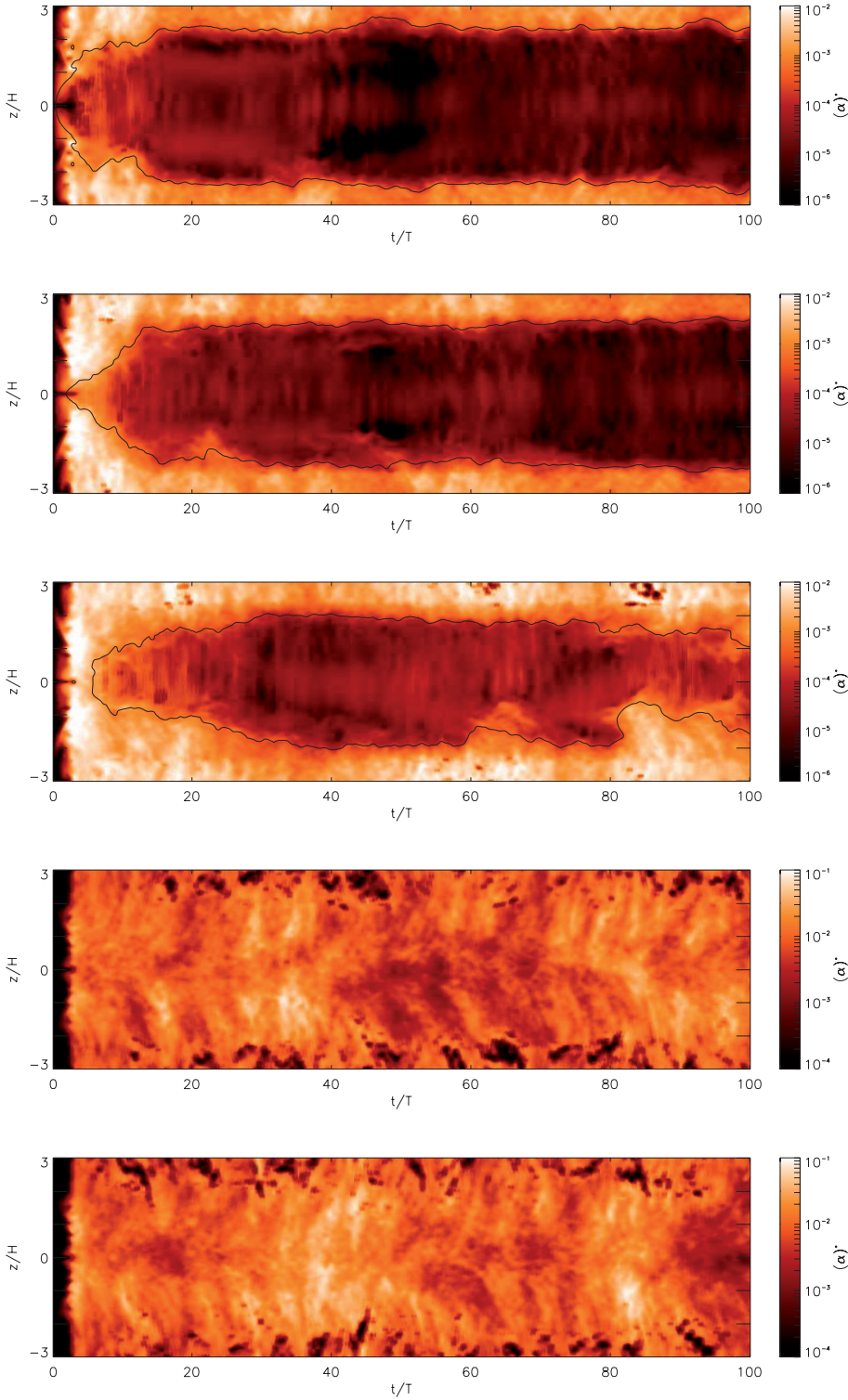
Fig. 7. mode12: Space-time plots of the horizontally averaged value of \alpha calculated at different radial positions R and a metal elemental abundance of x_{\text{Mg}} = 5 \times 10^{-11} . The cylindrical radius R varies from 1 AU ( top panel ) to 10 AU ( bottom panel ) passing through R = 3, 5, and 7 AU. The solid line drawn at the boundary between the live and dead zones indicates the position where the horizontally averaged Lundquist number Lu = 1 .
